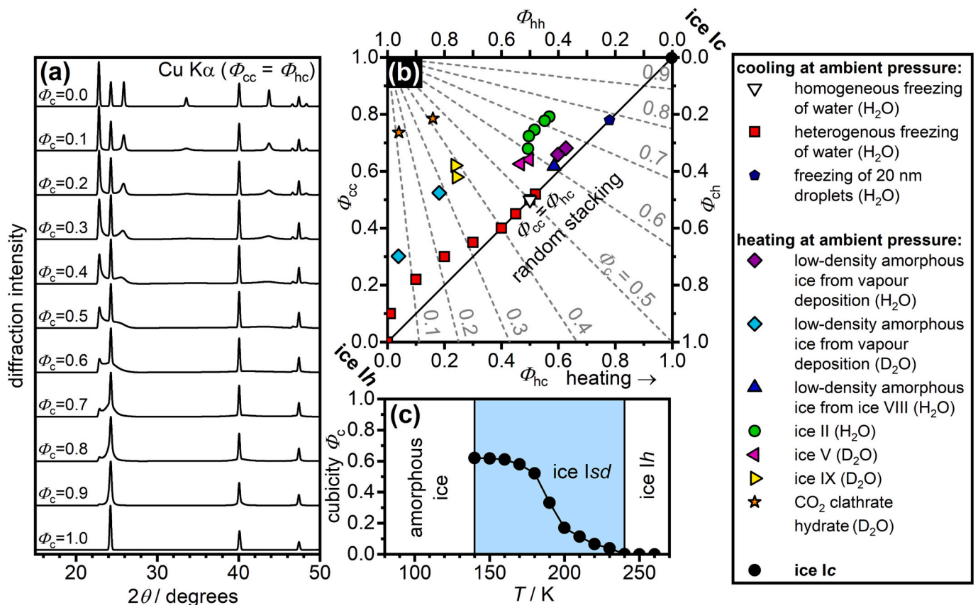
Fig. 2. (a) X-ray diffraction patterns (Cu K \alpha ) calculated with MCDIFFaX for ice I structure with cubicities, \Phi_c , from 0 to 1 and random stacking. (b) ‘Stackogram’ plot describing the structures of ice Isd by including first-order memory effects. The diagonal solid line indicates random stacking. Lines of constant \Phi_c are shown as dashed grey lines. The formation procedures of the ice Isd samples are indicated in the legend with data taken from (Amaya et al., 2017; del Rosso et al., 2020; Halukeerthi et al., 2020; Komatsu et al., 2020; Kuhs et al., 2012; Malkin et al., 2012; Malkin et al., 2015; Shephard et al., 2016; Talewar et al., 2019). (c) \Phi_c of H_2O ice Isd obtained by crystallising vapour-deposited amorphous ice (amorphous solid water) upon heating at ambient pressure (Rosu-Finsen et al., 2022).
