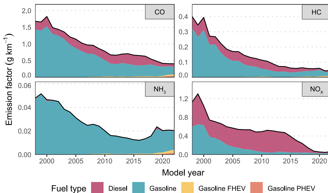
Fig. 4. Average passenger car distance-based emission factor values ( \text{g km}^{-1} ) as a function of model year for CO, HC, NH 3 , and NO x . The solid black line represents the average distance-based emission factor values and the shaded areas represent each fuel type's contribution towards the average.
