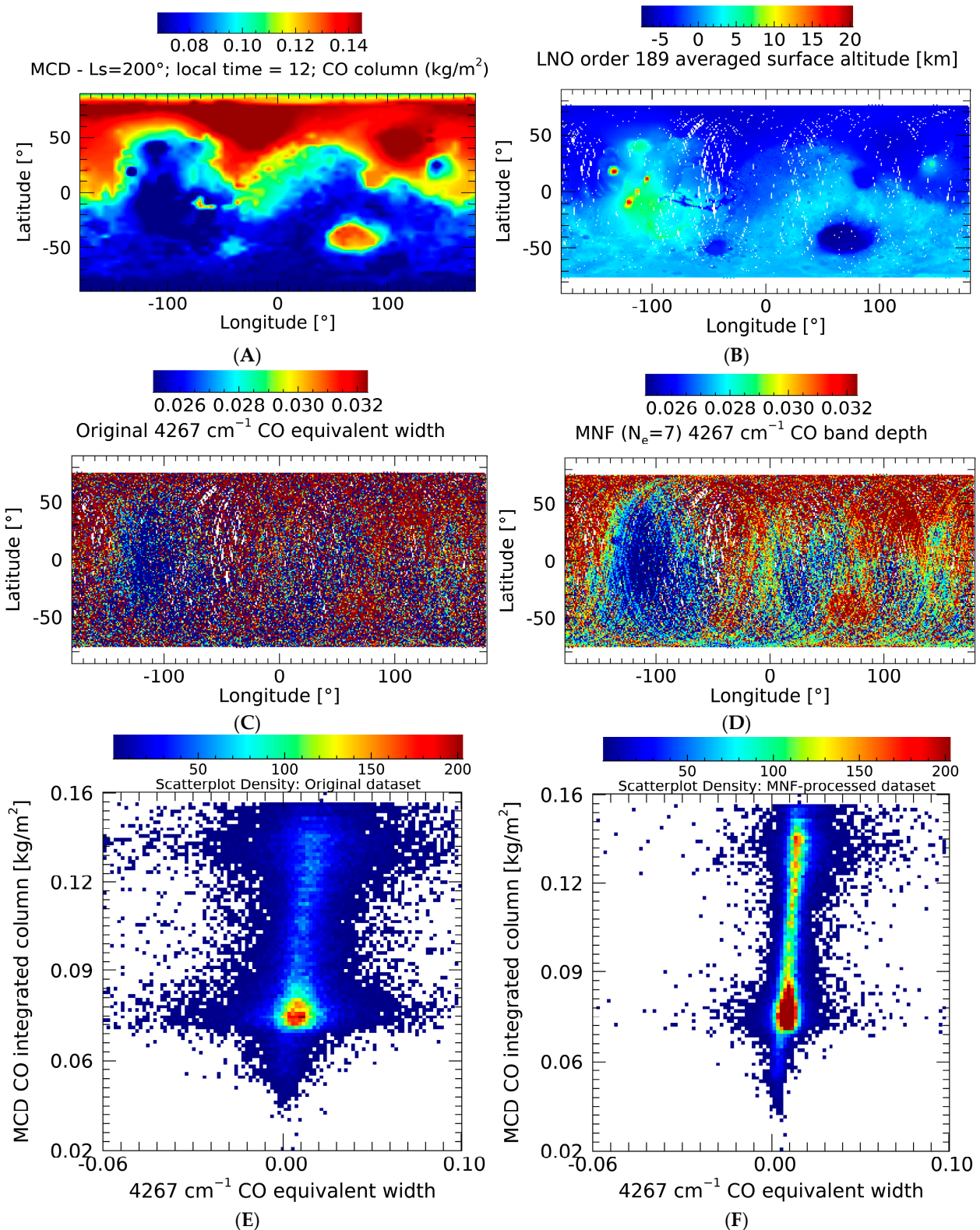
Figure 9. (A) MCD simulation of the CO-integrated column in \text{kg}/\text{m}^2 . (B) LNO order 189 averaged surface altimetry in km (from MOLA data, [37]). (C) Equivalent width of the CO 4267 \text{ cm}^{-1} absorption line computed on LNO order 189 original data. (D) Equivalent width of the CO 4267 \text{ cm}^{-1} absorption line computed on the MNF-processed data ( N_e = 7 ). (E) Density scatter plot of the quantities in panels (A,C). (F) As in panel (E), but here the quantities in panels (A,D) are being compared.
