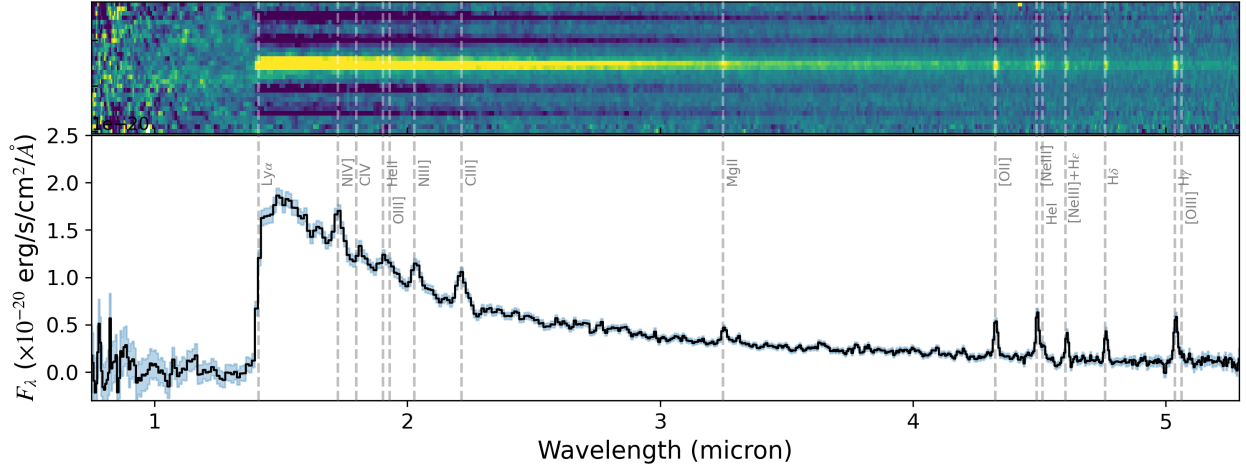
Fig. 2. 2D (top) and 1D (bottom) spectra of GN-z11 using the PRISM/CLEAR configuration of NIRSpc. The 1D spectrum has been extracted using a 3-pixel-wide aperture that leads to improved S/N in this highly compact object. Prominent emission lines present in the spectra are marked. The S/N of the continuum is high, and the emission lines are clearly seen in both the 1D and 2D spectra.
