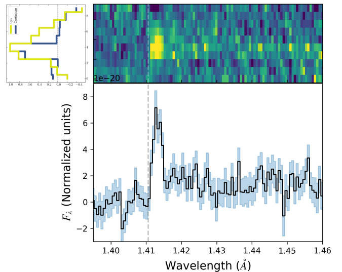
Fig. 6. Zoom in on the Ly \alpha emission line in the G140M 1D (lower) and 2D (upper) spectra. The dashed grey line shows the systemic wavelength of the Ly \alpha transition. The histograms (top left) of the Ly \alpha spatial profile (yellow) and that of the continuum (blue) show the Ly \alpha emission from GN-z11 is more extended towards the south-west (up in the MSA shutter in this view).
