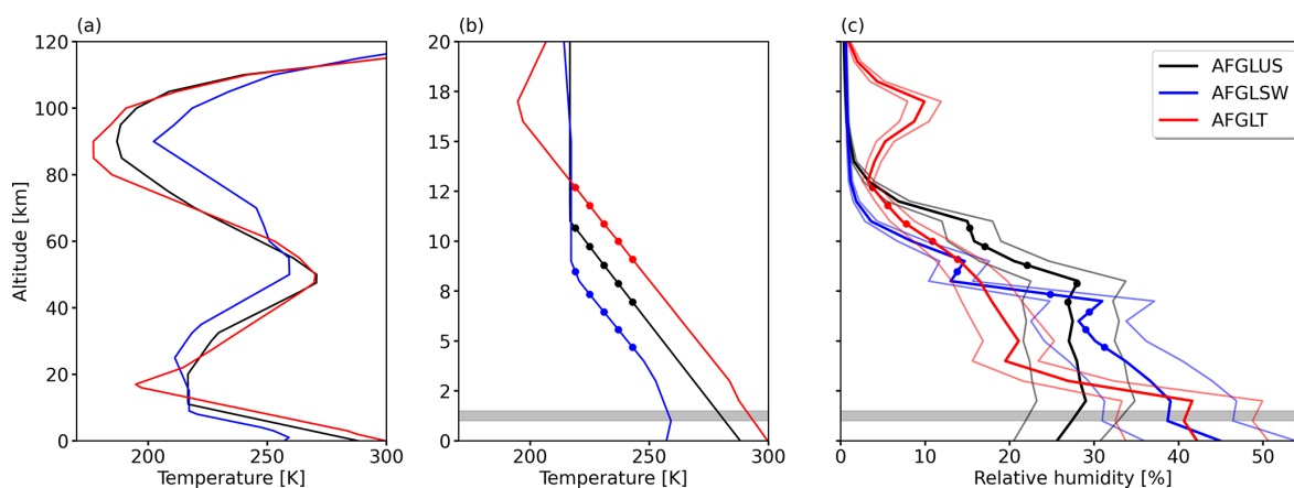
Figure B1. Profiles of temperature ( a , b ) and relative humidity ( c ) used for the radiative transfer simulations. The sub-Arctic ( afglsw ), mid-latitude ( afglus ), and tropical ( afglt ) profiles are given in blue, black, and red, respectively. The modified profiles with \pm 20\% are indicated by pale colors. The positions of the simulated ice water cloud are indicated by the colored dots for each profile. The position of the low-level liquid water cloud is indicated by the gray shaded area.
