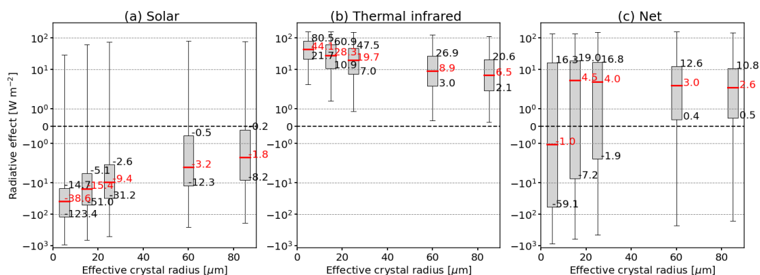
Figure 9. Same as Fig. 5 but as a function of effective crystal radius r_{\text{eff}} (in μm).
