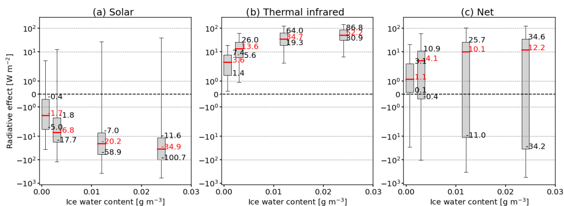
Figure 8. Same as Fig. 5 but as a function of ice water content IWC (in g m -3 ). For better legibility, only IWC values up to 0.03 g m -3 are plotted.
