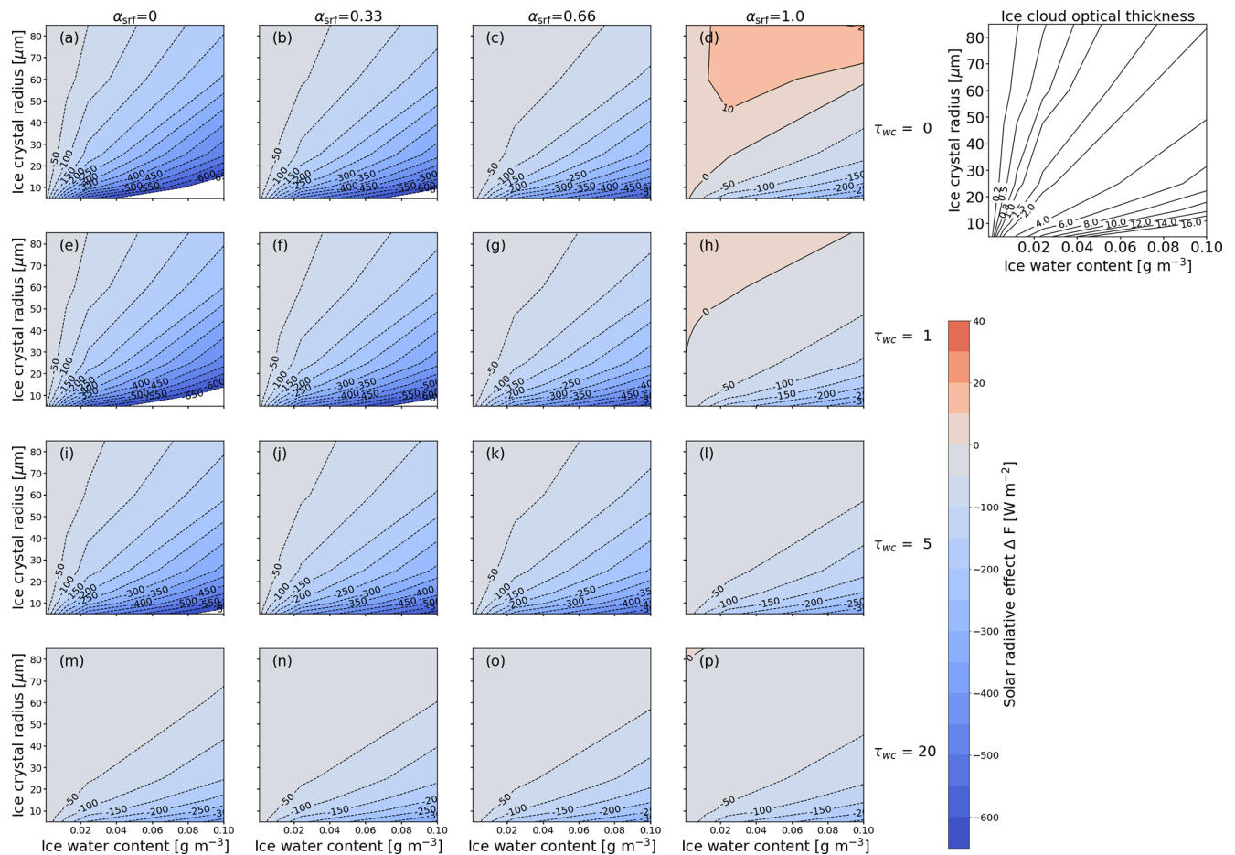
Figure 16. Same as Fig. 10 but \Delta F_{sol} (in W m^{-2} ) and combinations of surface albedo \alpha_{srf} and cloud optical thickness \tau_{liq} of the underlying liquid water cloud.
