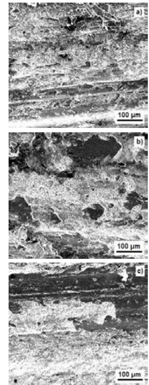
FIGURE 9. Worn surfaces at loads of a) 40 N, b) 90 N, c) 140 N.
