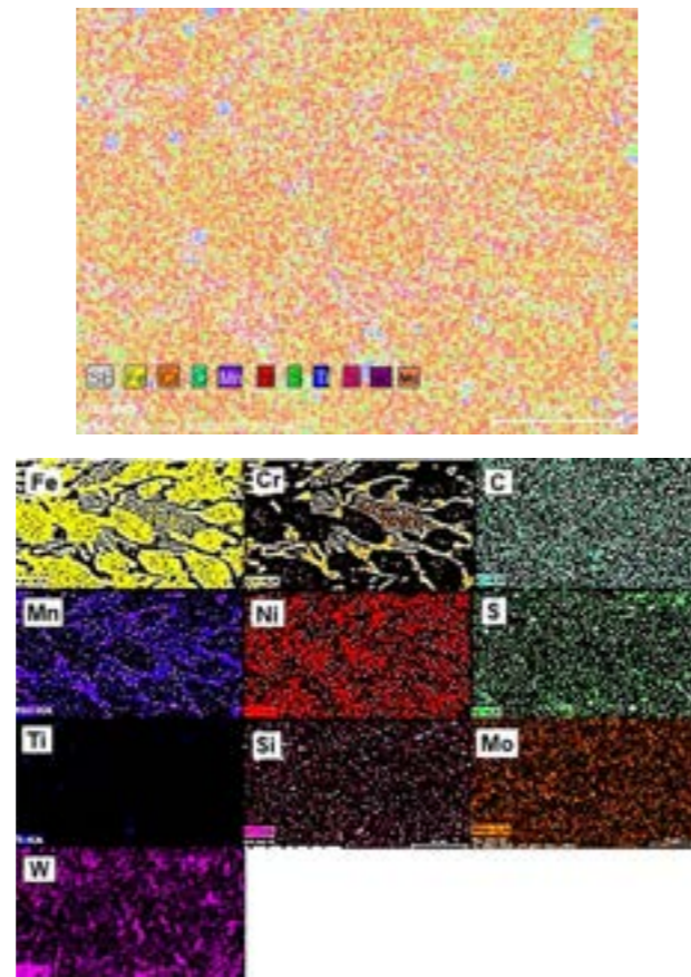
FIGURE 6. SEM mapped image analysis of sample S5.
