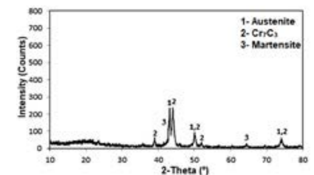
FIGURE 4. X-ray pattern of sample S5.
