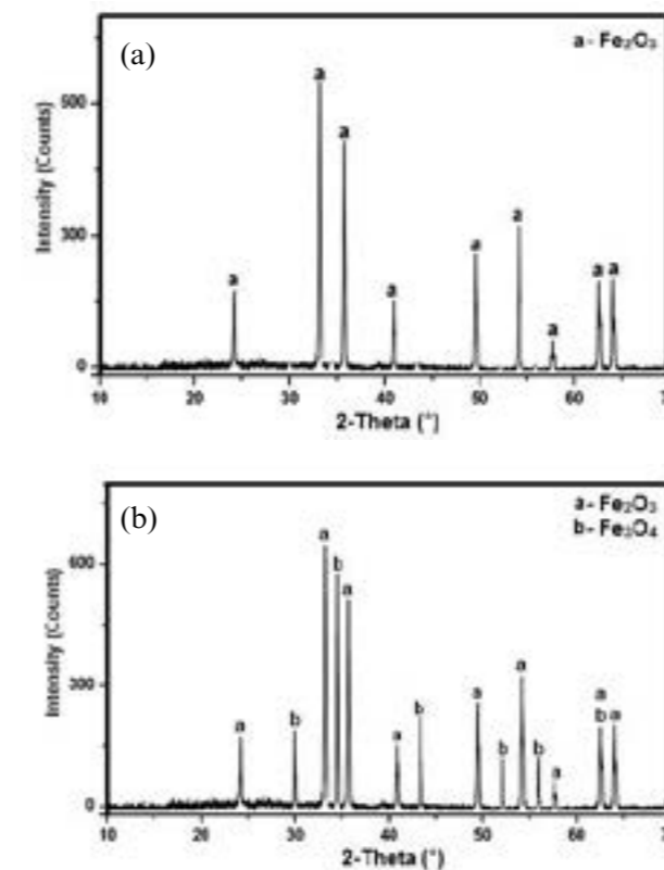
Figure 11. XRD patterns of worn particulates obtained from surface of sample S5.
