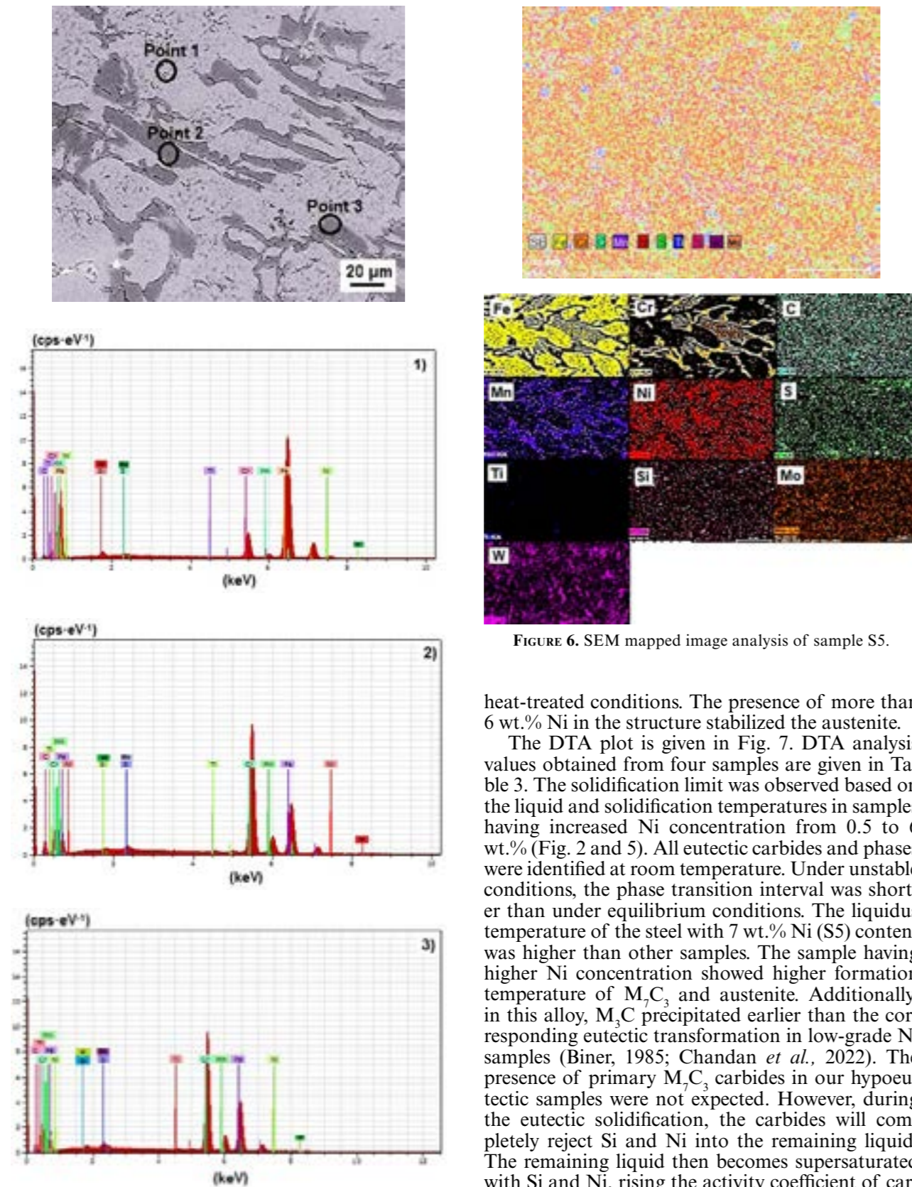
FIGURE 5. Chemical composition clarified by EDS of sample S5.
