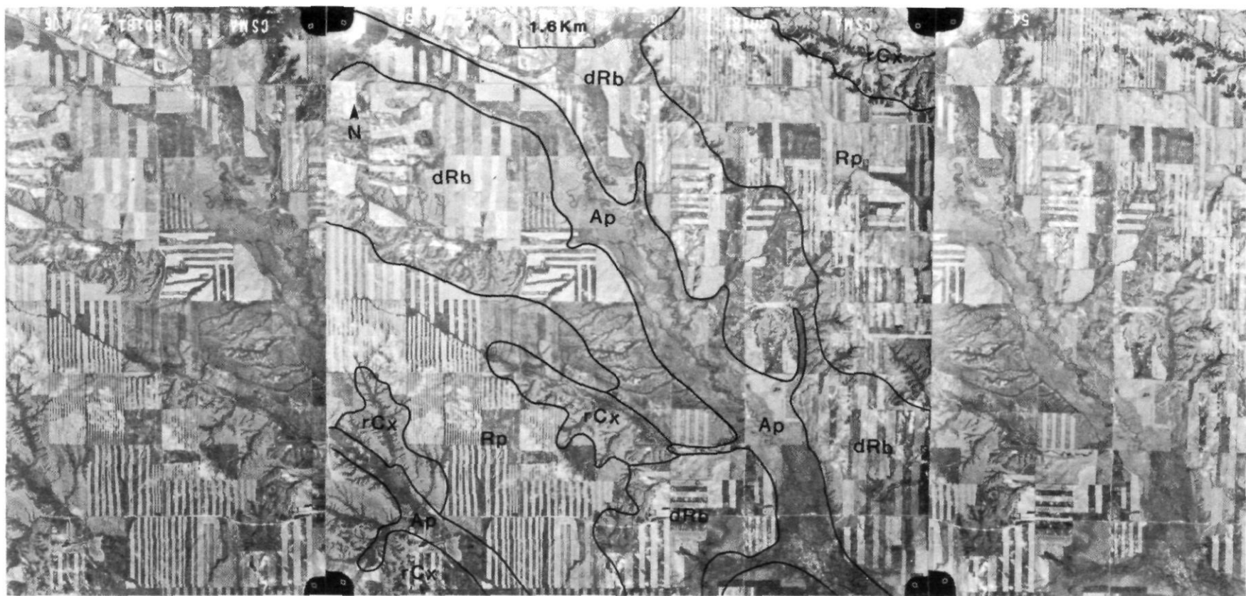
FIGURE 9. Stereo-triplet of southeast part of Wood Mountain area, showing unglaciated bedrock (Rp), gentle slopes (dRb), and alluvial plains (Ap) of Poplar River valley (centre) and Bolster Creek (left corner). Centre of figure is Sec. 22, tp. 2, rge. 1 (49°08'N, 106°04'W). Airphotos CSMA 80181-06-12-54, 56, 58.
