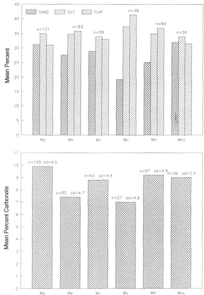
FIGURE 21. Textural characteristics (upper graph) and carbonate contents of the silt fraction (lower graph) of tills and diamictons associated with morainic map units in the Cypress Lake and Wood Mountain areas. See Figure 5 for explanation of letter symbols.
