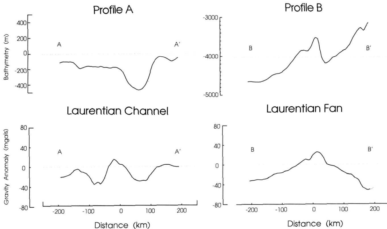
FIGURE 5. Profiles of gravity and bathymetry along lines A and B shown in Figure 2a and b.
