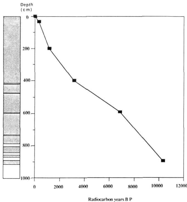
FIGURE 2. Core depths plotted versus radiocarbon age for the core. A date of 330 yr BP was assigned to the rise of ragweed pollen percentages near the top of the core, and a date of 0 yr BP was assigned to the top of the core. Lithology of the core included: stippled pattern indicates sand bodies; cross-hatched pattern indicates organic-rich sediments (gyttja).
