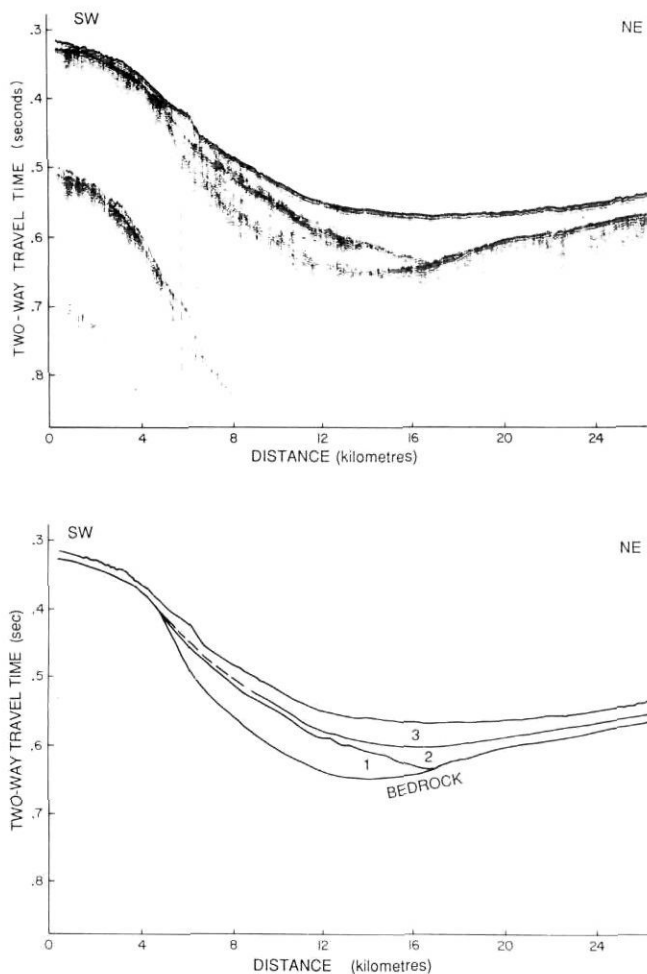
FIGURE 10. Section G — airgun seismic profile illustrating sediment relationships where the western basin was diagonally intersected east of the Core 68 locality. Unit 1 is confined to the area on and adjacent to the southern flank of the basin (see Fig. 1 for location).
