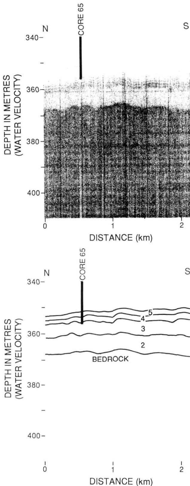
FIGURE 11. Hunttec high resolution profile showing the Quaternary sediment units at core locations 65 southwest of Charles Island.
