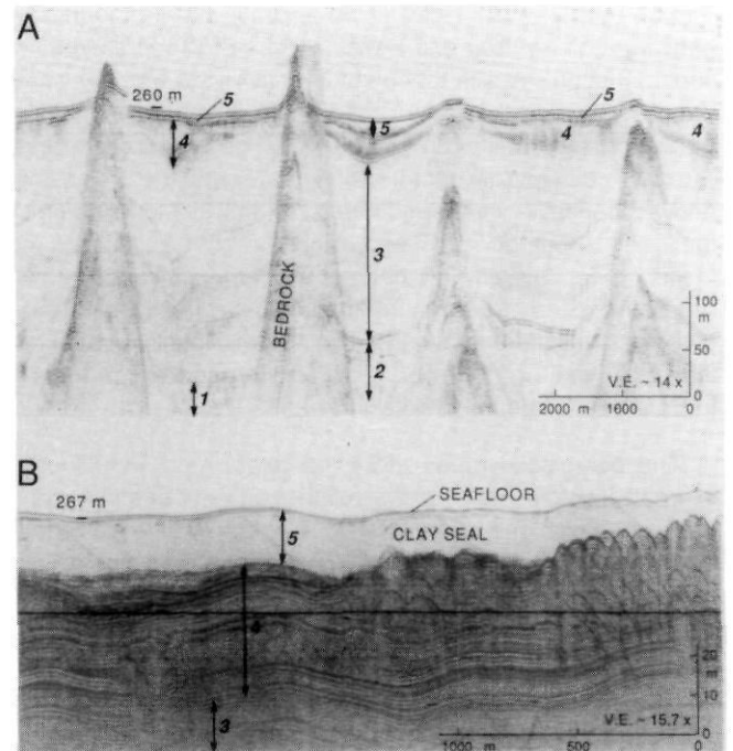
FIGURE 10. Examples of the world's largest internal slump within the paraglacial deltaic sediments of the lower portion of the Saguenay Fjord: A: airgun record of three traverses of the fjord, showing variable failure within the unit; B: Huntec record shows the complexity of failure within unit 4 and the overlying clay of unit 5.
