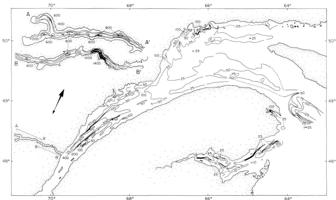
FIGURE 12. Isopach of total Quaternary sediment thickness within the St. Lawrence Estuary and adjacent seas.
