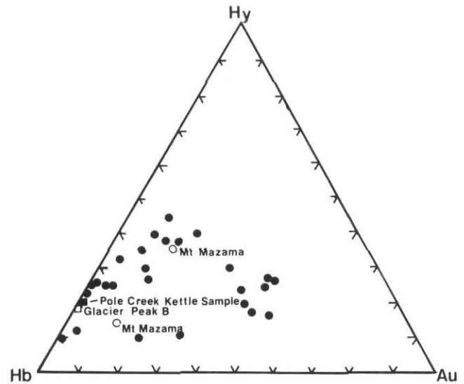
FIGURE 3. Petrographically determined proportions of Hornblende, Hypersthène and Augite of non-Cummingtonite bearing tephra found in the White Cloud Peaks — Boulder Mountains study area and correlative Cascade Range Reference samples. Including: Mount Mazama (Reference samples = open circles, Idaho samples = closed circles); and Glacier Peak — Set B (Reference sample = open square, Idaho sample = closed square) tephra.
