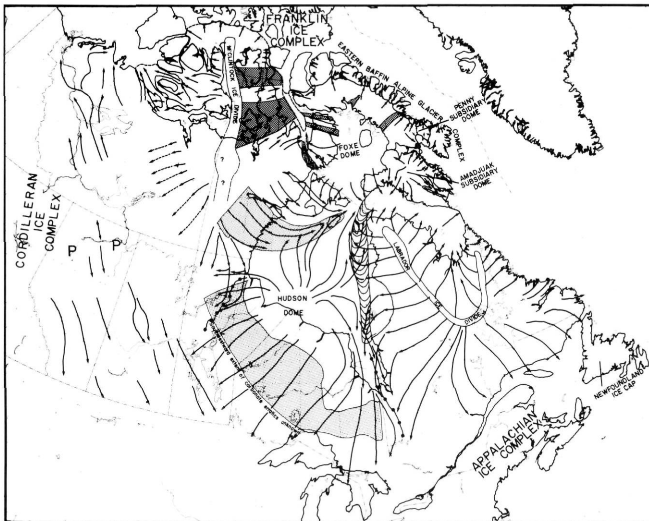
FIGURE 4. The structure and dynamics of the Laurentide Ice Sheet during the Late Wisconsinan maximum, from DYKE et al. (1982).
