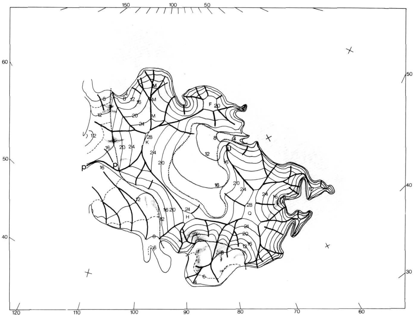
FIGURE 3. Computer reconstruction of the Laurentide Ice Sheet at 18 ka with deformable Hudson Bay, Prairie and Great Lakes beds. Surface elevations are in 100's of metres above present sea level. Lettered features are as in the caption of Figure 2. Ice flow lines are perpendicular to the elevation contours. Heavy lines denote ice divides and dotted lines mark the boundary between hard and deformable beds.
