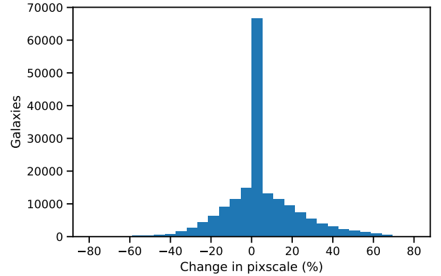
Figure B3. Change in resized pixel scale (pixscale), proportional to field-of-view in the final resized RGB images. The vast majority of galaxies have a tractor-estimated pixel scale within 20% of the pixel scale they would have had if we had access to NSA Petrosian radii. They would therefore have similar fields-of-view to GZ DECaLS galaxies, ensuring our DECaLS-derived labels remain applicable.
