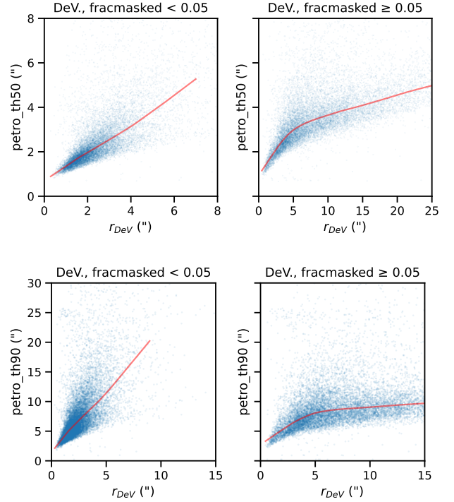
Figure B2. As with Fig. B1, but for tractor sources reported as having DeV-dominated light profiles. r_{DeV} is the half-light radius of the r-band DeV profile reported by tractor. Empirical relationships are fit separately for galaxies with over 5% tractor-masked pixels ( fracmasked ), as these follow a qualitatively different relationship.
