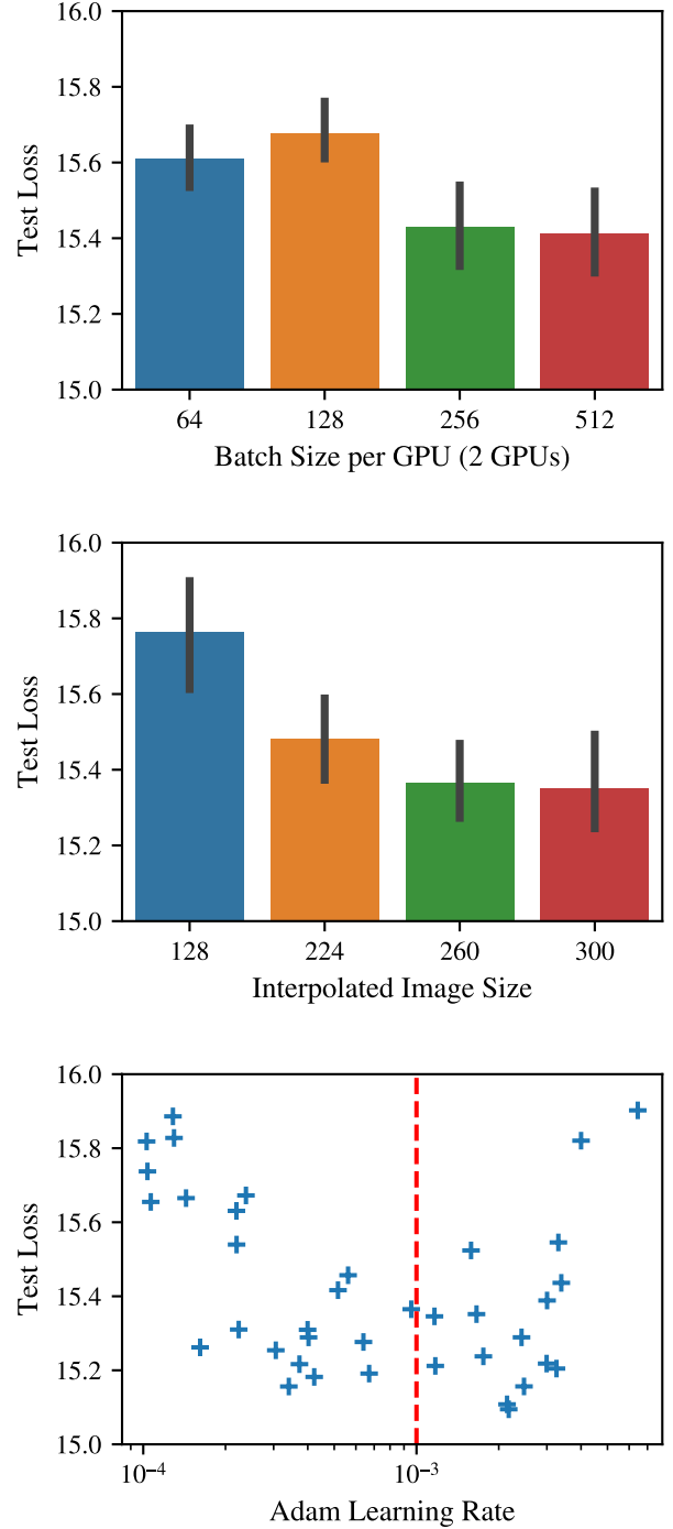
Figure C1. Architectural hyperparameter search results for batch size (upper), image size (middle), and learning rate (lower). Larger batch sizes and larger images are likely helpful. The ideal learning rate is likely close to the conventional 10^{-3} value.
