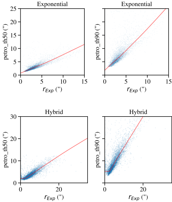
Figure B1. Estimating SDSS/NSA radii measurements from DESI-L/tractor measurements, for tractor sources reported as having exponential-dominated or hybrid light profiles. r_{Exp} is the half-light radius of the r-band exponential profile reported by tractor, while petro\_th50 and petro\_th90 are the 50% and 90% Petrosian radii reported by the NSA. Blue points are galaxies with both tractor and NSA measurements, and red curves are the resulting nonparametric LOWESS fit (local sampling fraction of 0.3).
