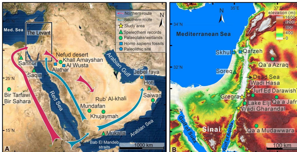
Fig. 1. Map showing archaeological, paleoclimatological, and paleoenvironmental records from the Levant and Arabia mentioned in the text. (A) The arrows indicate the suggested routes of human dispersals out of Africa [see (9, 17)]. The blue squares show sites with human fossils and footprints in northern Arabia, including those at Al Wusta paleolake (4) and Alathar paleolake (16), respectively. The green circles refer to paleolake/wetland sediments in the western desert of Egypt and Arabia, namely: Bir Tirdawi and Bir Sahara (52), Khall Amayshan (21), Mundafan (22), Khujaymah (22), and Saiwan (60). The green triangles show speleothem deposition in caves in the eastern desert of Egypt, including Saqia cave (43), Wadi Sannur (45), and in southern Arabia including Hoti cave in Oman and Mukkala cave in Yemen (23, 59). The main dated archaeological site in southeastern Arabia is Jebel Faya in the UAE (blue rhombus) (24, 58). (B) Digital elevation model map of the Levant showing the location of the study areas (yellow stars) along the Jordan Rift Valley (Wadi Gharandal and Gregra) and in the Jordanian Plateau (Wadi Hasa), and the paleolakes and speleothem records in the region. Paleolakes are represented by green circles, namely: Qa'a Azraq (53), Jurf Ed Darawish (26, 32), Lake Elji (54), Qa'a Jafr (27, 55), and Qa'a Mudawwara (28). Speleothem records in the Levant include Soreq cave (green triangle) (44, 46), and the blue squares show sites with human fossils including Skhul and Qafzeh caves (5). The source of digital elevation model data is derived from www.gslcloud.cn .
