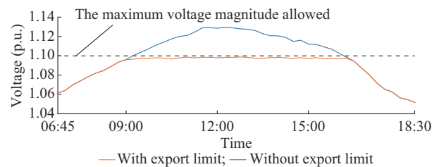
Fig. 10. Voltage magnitude of user 179 with and without export limit in a scenario of high irradiance and low consumption simulated in OpenDSS.
