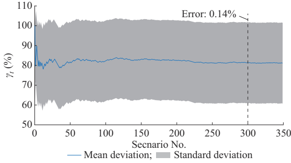
Fig. 6. Convergence of mean and standard deviations of \gamma_i for time step at 12:30 for Monte Carlo simulation.
