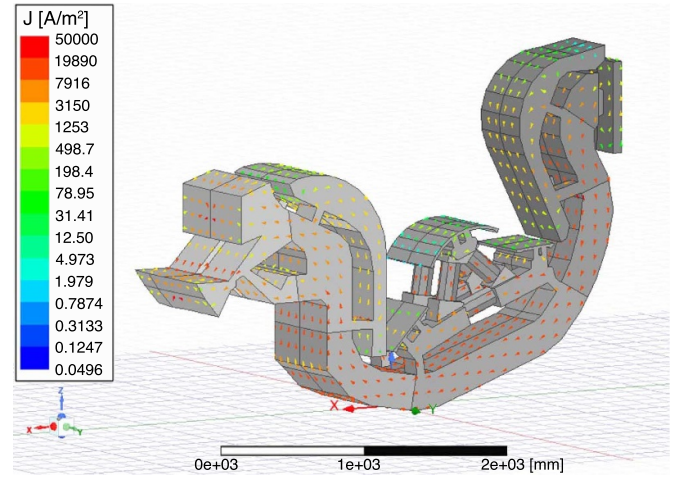
Figure 7. ANSYS ® Maxwell electric transient FEM simulation of the simplified CAD model. About 1 kA is applied to the inboard vacuum vessel connection vessel surface and the outboard vacuum vessel connection is defined as the ground terminal. The field overlay for the peak j_{||} of the simulation demonstrates the path of current flow along the divertor cassette body.
