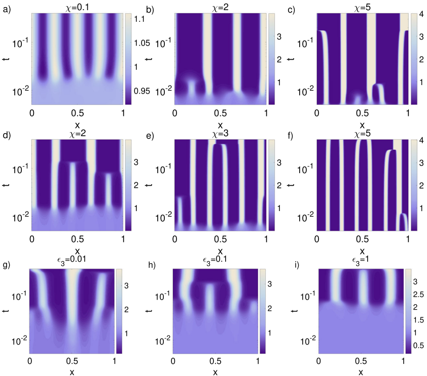
Fig. 10 1D simulations for the time scale of pattern formation. a–c The 1D cell concentration for parameters in Fig. 9a, \epsilon_2 = 1 , and varying \chi \in \{0.1, 2, 5\} . d–f The 1D cell concentration for parameters in Fig. 9b, \epsilon_2 = 1 and varying \chi \in \{2, 3, 5\} . g–i The 1D cell concentration for parameters in Fig. 9c, \chi = 4 and varying \epsilon_3 \in \{0.01, 0.1, 1\} . Note the different scaling of the colorbar, and that the time axes are displayed in logarithmic scale (Color figure online)
