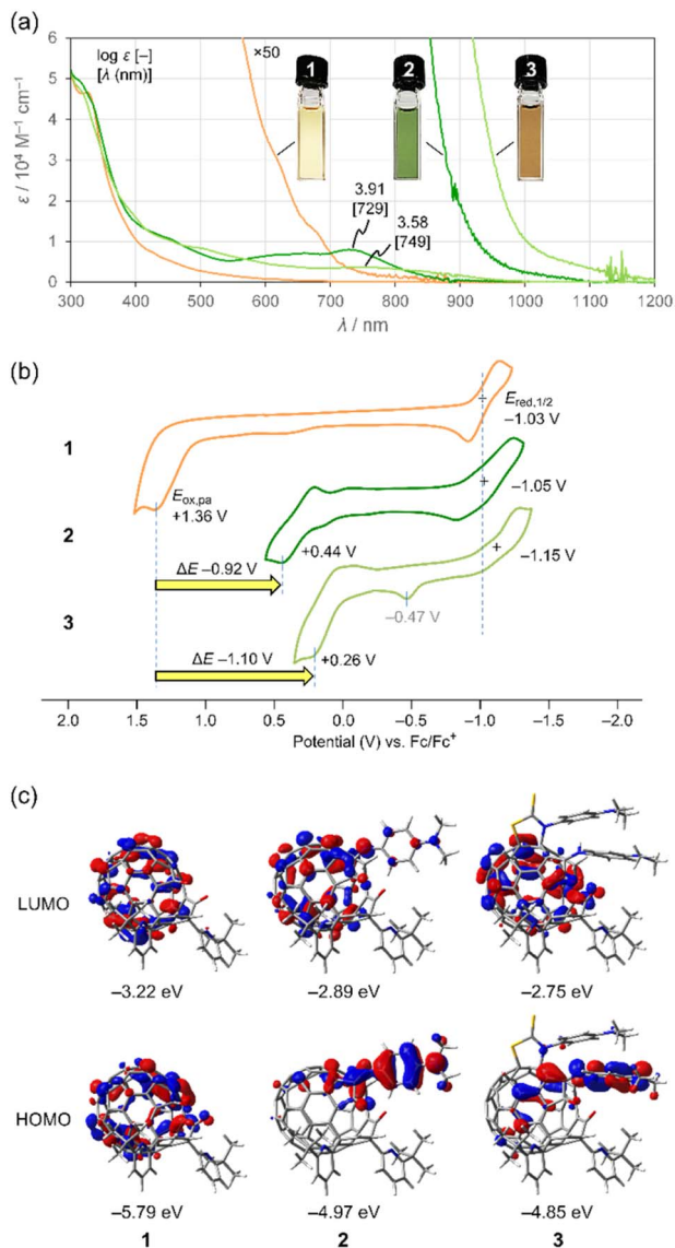
Fig. 5 (a) UV-vis-NIR absorption spectra of 1–3 (50 μM in benzene). (b) Cyclic voltammograms of 1–3 (1 mM in ODCB, 0.1 M n -Bu 4 N·BF 4 , 100 mV s -1 ). (c) Molecular orbitals of 1–3 (B3LYP-D3/6-31G(d)).
