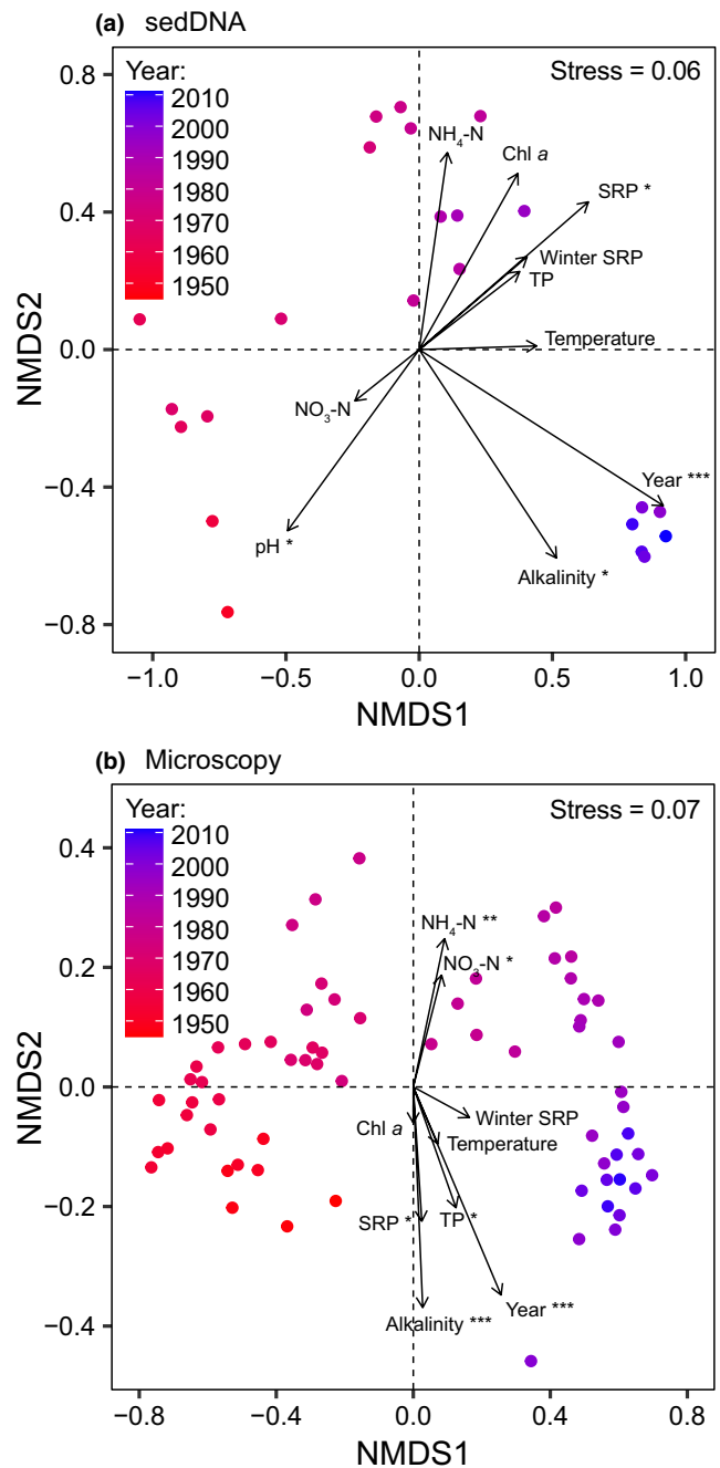
FIGURE 1 NMDS of a Bray–Curtis dissimilarity matrix based on beta diversity as measured by sedDNA (a) and microscopy (b) from 1945 to 2010. The red to blue gradient indicates older to more recent samples. Vectors for sample year and the lake physiochemical conditions that correlated with each dissimilarity matrix are fitted. Vector length is proportional to the strength of the correlation. *** p < .001 , ** p < .01 , * p < .05 . NMDS stress values are shown.
