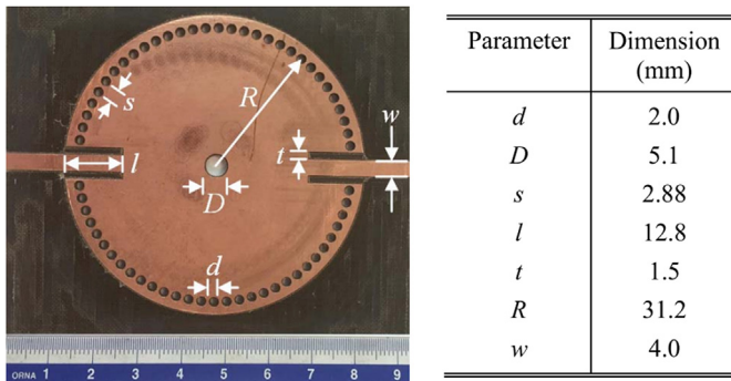
Fig. 5. Geometry structure of SIW cavity-type sensor [61].
