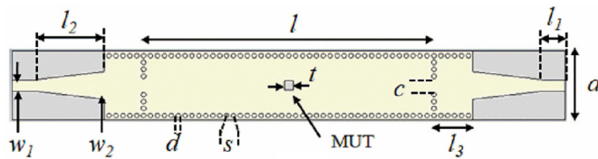
Fig. 6. SIW cavity-type microwave sensor using several high-order modes [62].
