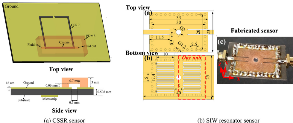
Fig. 7. Microwave sensor structure; (a) top and side view of the CSRR-type [64] (b) top, bottom, and fabricated views of the SIW resonator type [65].
