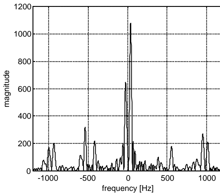
Figure 4. Estimated WVD of the space-phasor (signal in figure 1), at the time point t=0.06 s. (after the fault).
