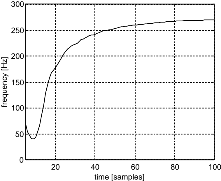
Figure 6. Estimated instantaneous frequency of the signal in figure 2.
