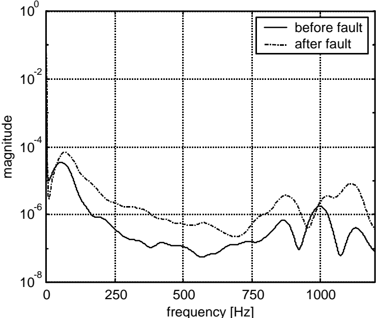
Figure 5. Power spectrum of the signal in figure 1.
