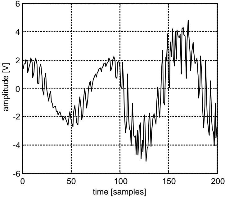
Figure 1. Voltage waveform (phase R) at the motor input during a short circuit. Fault occurs after the 100 th sample.
