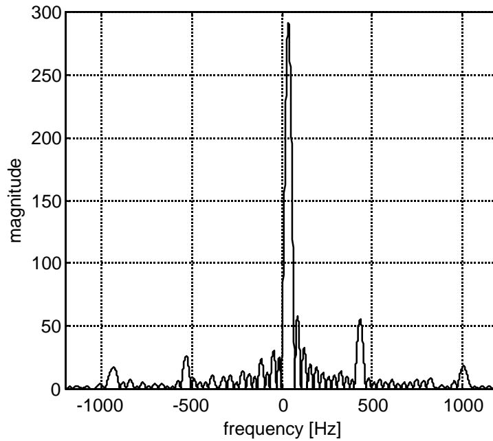
Figure 3. Estimated WVD of the space-phasor (signal in figure 1), at the time point t=0.015 s. (before the fault).
