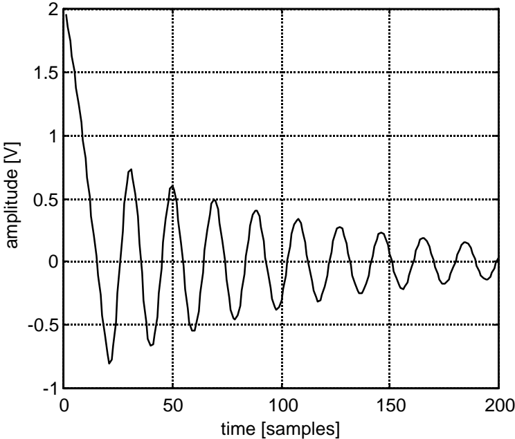
Figure 2. Voltage waveform (faulted phase) during single line to ground short circuit. Fault occurs after the 20 th sample.
