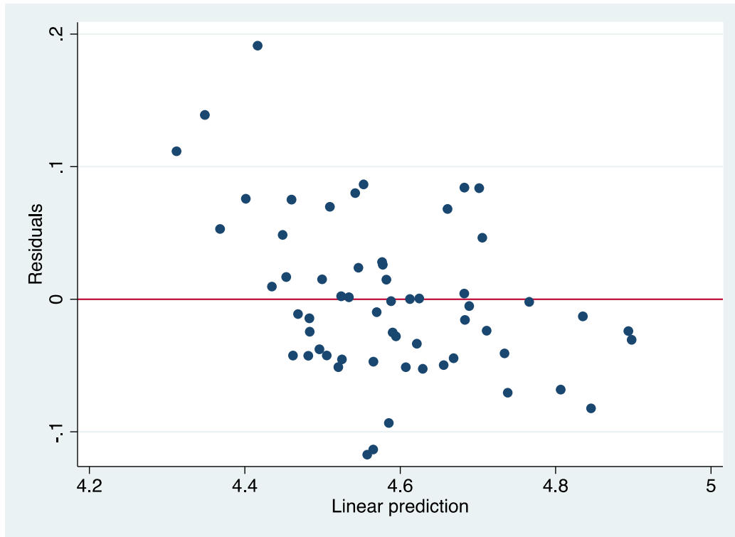
Fitted values Scattered Against Residuals with M2/GDP and U.S. Interest Rates
