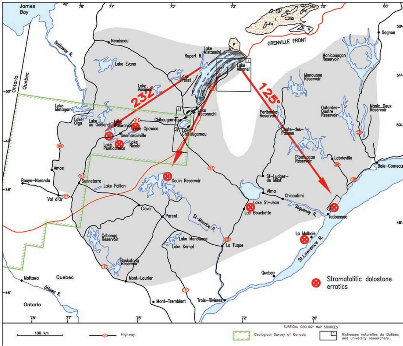
FIGURE 16. Dispersal of stromatolitic dolostone erratics from the Alabanel Formation.
