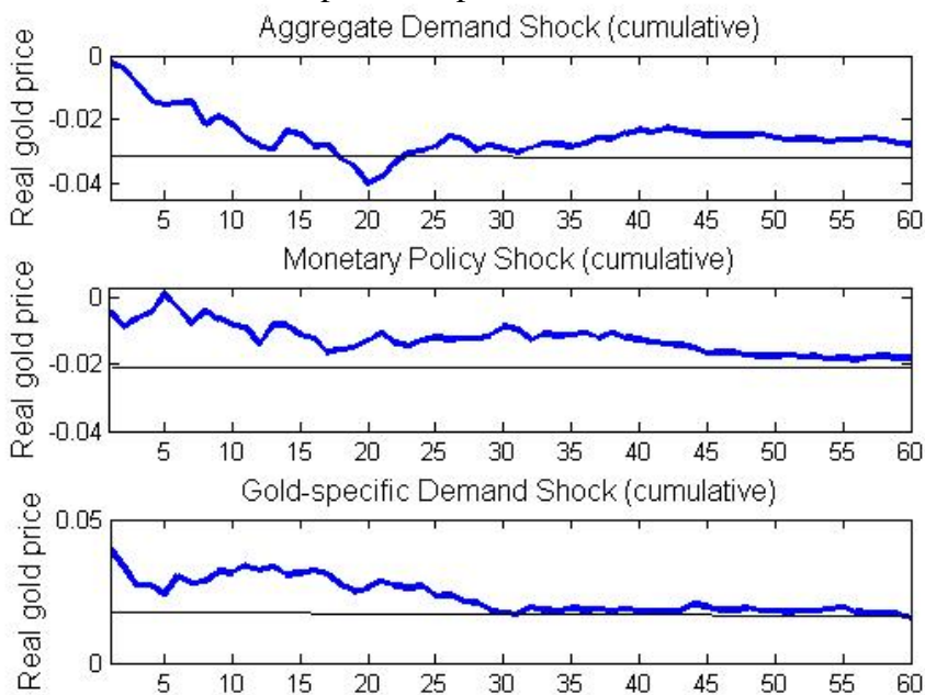
Figure 7 Cumulative Impulse Responses of Various Structural Shocks
