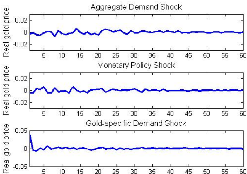
Figure 6 Impulse Responses of Various Structural Shocks
