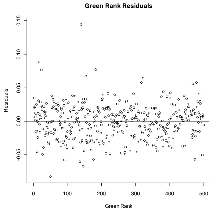
Figure 10: Residual Plot from Regression 2.
