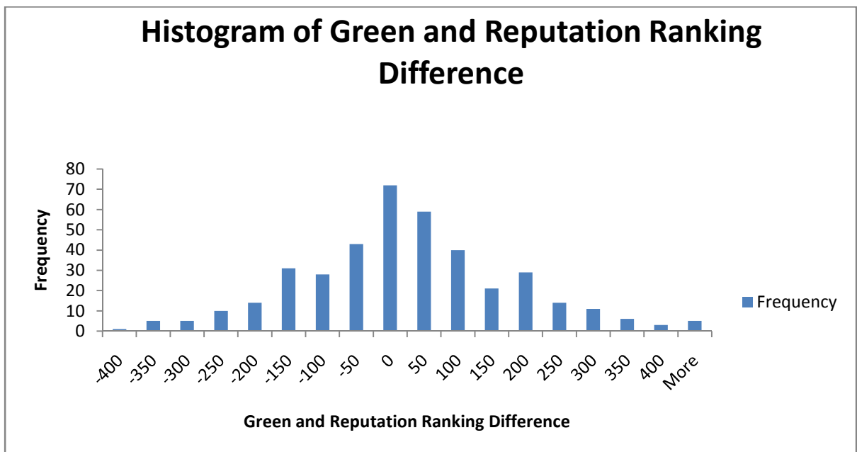
Figure 11: Green and Reputation Ranking Difference Histogram
