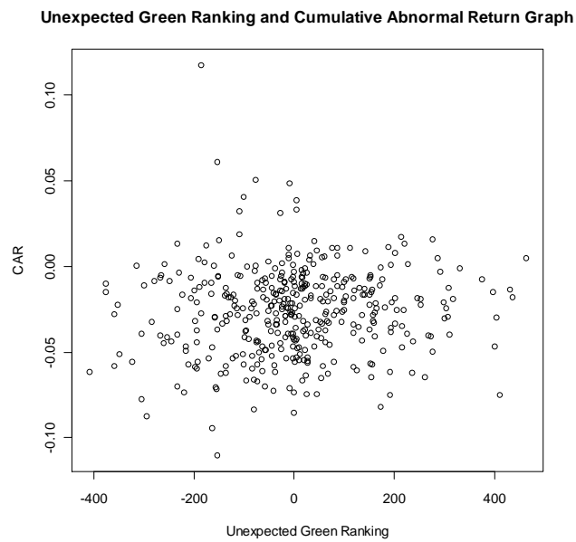
Figure 12: Scatter Plot Displaying Relationship of Regression 3.
