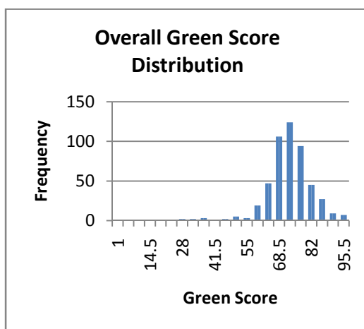
Figure 2: Green Score Histogram
