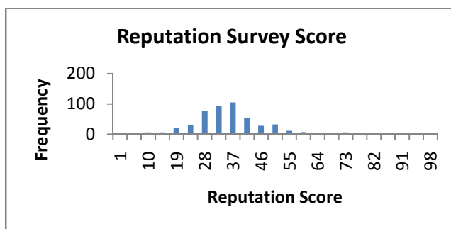
Figure 5: Reputation Score Histogram
