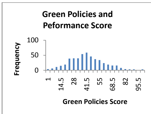
Figure 4: Green Policies and Performance Histogram
