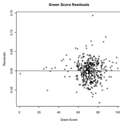
Figure 8: Residual Plot from Regression 1.
