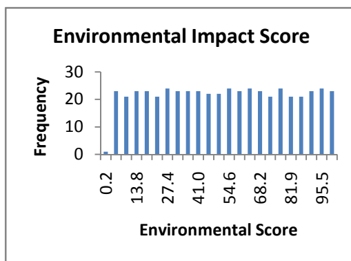
Figure 3: Environmental Score Histogram
