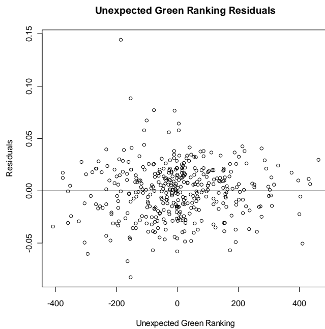
Figure 13: Residual Plot from Regression 3.
