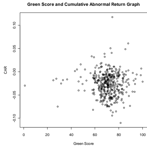
Figure 7: Scatter Plot Displaying Relationship of Regression 1.
