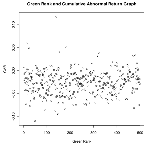
Figure 9: Scatter Plot Displaying Relationship of Regression 2.
