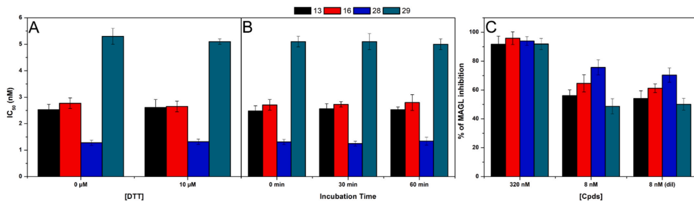
Fig. 3. Analysis of the mechanism of MAGL inhibition of compounds 13, 16, 28 and 29. A) Effect of DTT on MAGL inhibition activity. B) IC_{50} (nM) values at different pre-incubation times with MAGL (0 min, 30 min and 60 min). C) Dilution assay: the first two columns indicate the inhibition percentage of the compound at a concentration of 320 nM and 8 nM. The third column indicates the inhibition percentage of the compound after dilution (final concentration = 8 nM).
