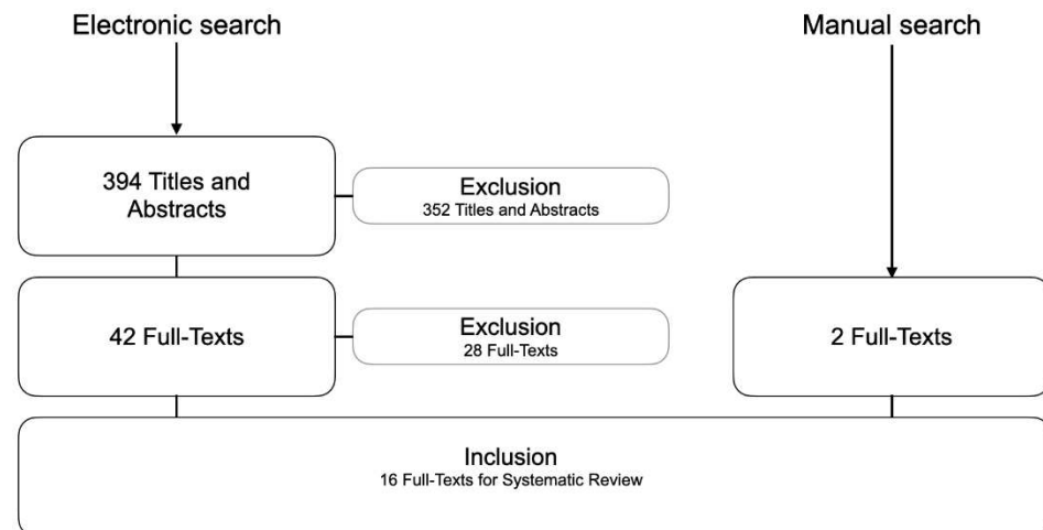
Figure 1. Flow-chart showing the electronic and manual search results.
