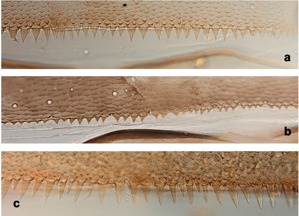
Figure 5. Larvae, posterior margins of terga VII a Centroptilum samraouii sp. nov. b Centroptilum alamaiae sp. nov. c Centroptilum luteolum .
