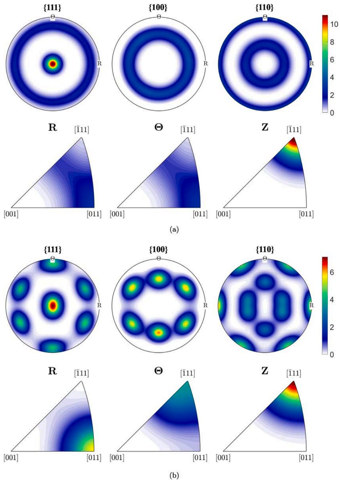
Fig. 9. Initial \langle 111 \rangle \parallel Z fiber texture. Microstructure N5000-D1. Pole figures for \{111\} , \{100\} and \{110\} plane families with respect to (R, \theta, Z) coordinate system, and inverse pole figures for R , \theta and Z directions with respect to [001] , [011] and \bar{1}11 crystallographic axes. Results corresponding to: (a) undeformed and (b) deformed configurations, respectively. The deformed configuration is computed at the necking time. The calculations are performed for a loading velocity V_R = 1000 m/s. (For interpretation of the references to color in this figure legend, the reader is referred to the web version of this article.)
