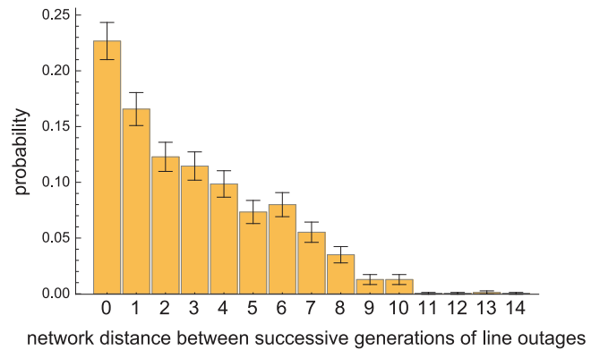
Fig. 4. Probability distribution of network distance d_{\text{mean}}^{\text{bus}}(G_i, G_{i+1}) between successive generations of line outages. The error bars show a 95% confidence interval.
