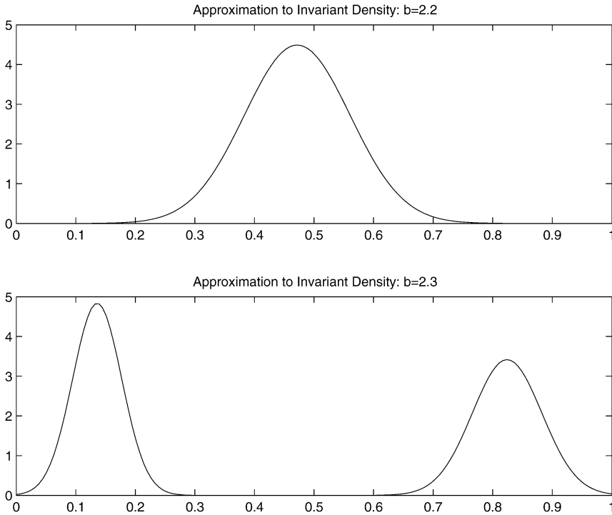
FIG. 4. Approximations from Theorem 2 for the limiting invariant densities of (3) in the case when f(x) = x + 1 - b \sin x . In the top, we take b = 2.2 so that f has stable fixed point x_s \approx 0.47 and in the bottom, we take b = 2.3 so that f has stable period two orbit P \approx \{0.14, 0.82\} .
