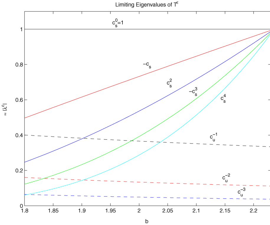
FIG. 1. Modulus of the top limiting eigenvalues of T^\epsilon as given by Theorem 1 plotted against b up to the first period doubling bifurcation point at b = \sqrt{5} \approx 2.23 . The solid lines are powers of c_s while the dashed lines are negative powers of c_u .
