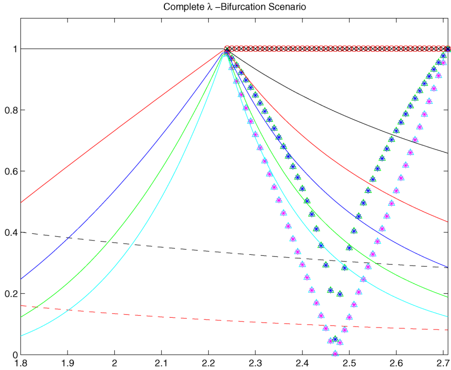
FIG. 3. Illustration of \lambda -bifurcation scenario for f(x) = x + 1 - b \sin x , 1.8 < b < 2.71 . See also Figures 1 and 2.
