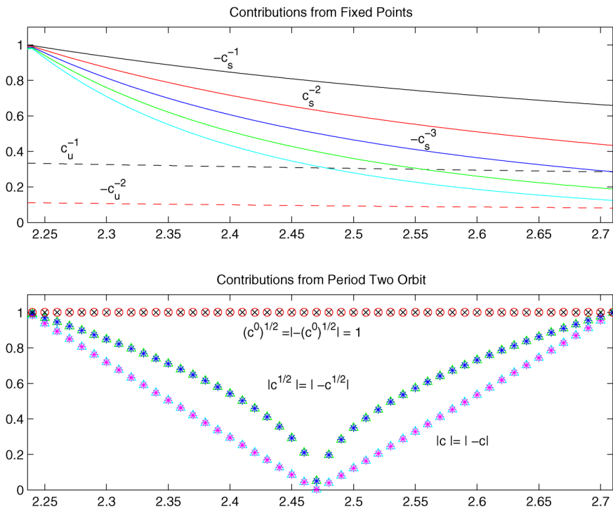
FIG. 2. Modulus of the top limiting eigenvalues of T^\epsilon as \epsilon \rightarrow 0 as given by Theorem 1 plotted against b between the first period doubling bifurcation point at b = \sqrt{5} \approx 2.23 and the second near b \approx 2.71 .
