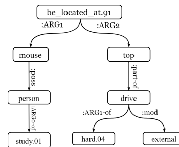
Figure 1: The AMR graph for the English text “The student’s mouse is on top of the external hard drive”.
