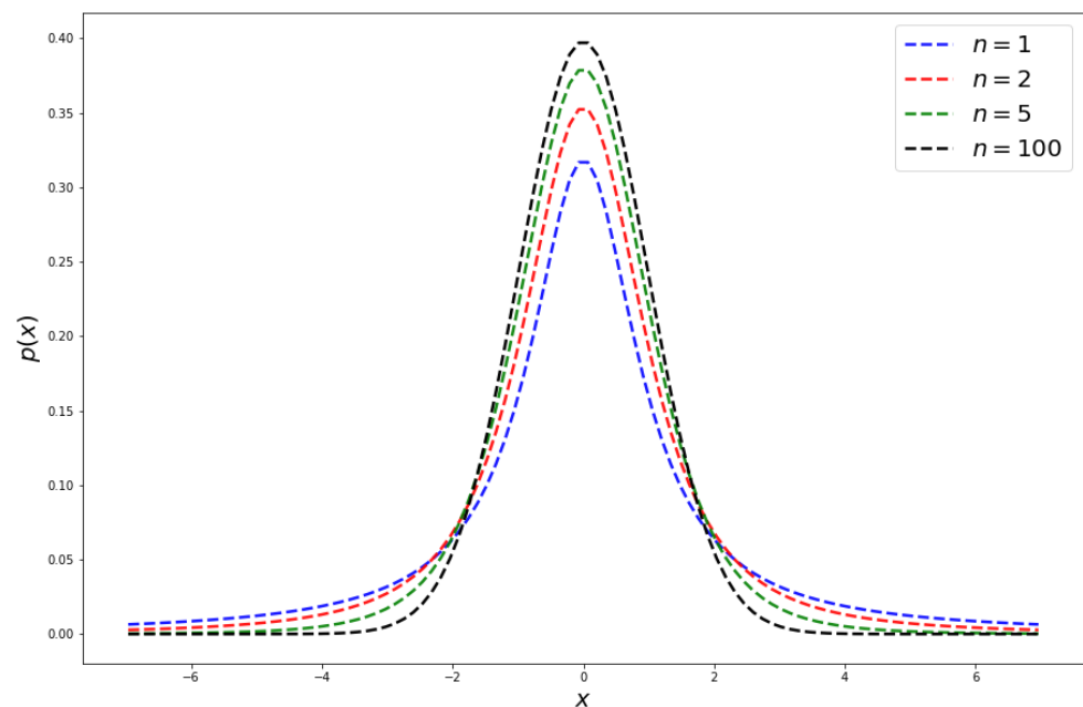
Figure 1. Student’s t distribution, Equation (9), for different degrees of freedom n .
