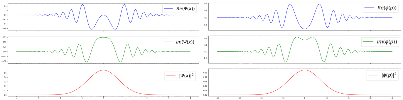
Figure 2. Examples of wavefunction (14) and (15): real (top) and imaginary (middle) parts and square modulus (bottom).
