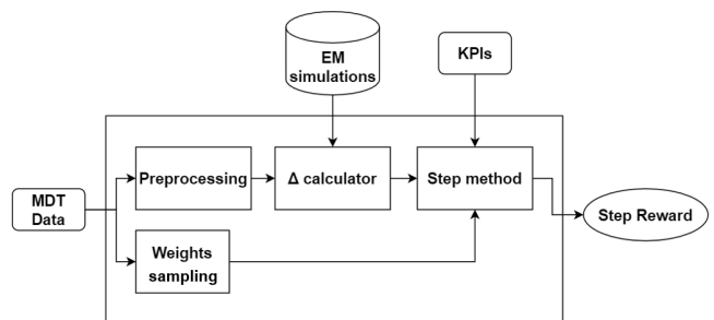
Fig. 4: Simulated environment - block system view
