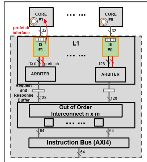
Fig. 7: Two-level cache with L1 prefetch after IF optimization with 4x32bit ring FIFO buffer and additional conditional branch pipeline. Critical path is shown by the red arrow.
