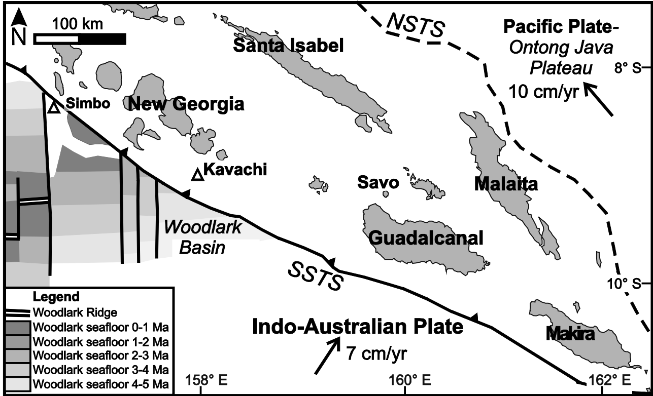
Fig. 1: Map of the Solomon Islands showing major tectonic features, and locations discussed in the text. Woodlark seafloor ages from Taylor (1987). Plate motions from Petterson et al. (1999).
