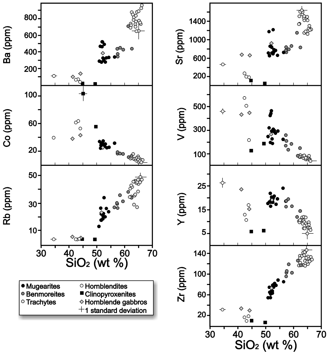
Fig. 7: Selected trace element Harker variation diagrams for main suite and nodule samples from Savo Island. SiO 2 from major element analyses, recalculated to 100% on a volatile-free basis. Error bars show typical precision (1 standard deviation).
