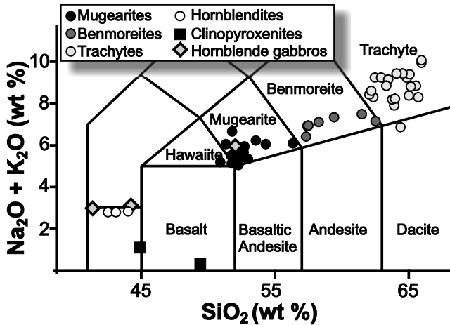
Fig. 2: Total alkalis vs. silica for samples from Savo (after Le Maitre et al. 1989). Samples recalculated to 100% on a volatile-free basis. Samples are sodic ( \text{Na}_2\text{O}-2>\text{K}_2\text{O} ), contain less than 20% normative quartz, and are thus classified as a hawaiiite–trachyte series.
