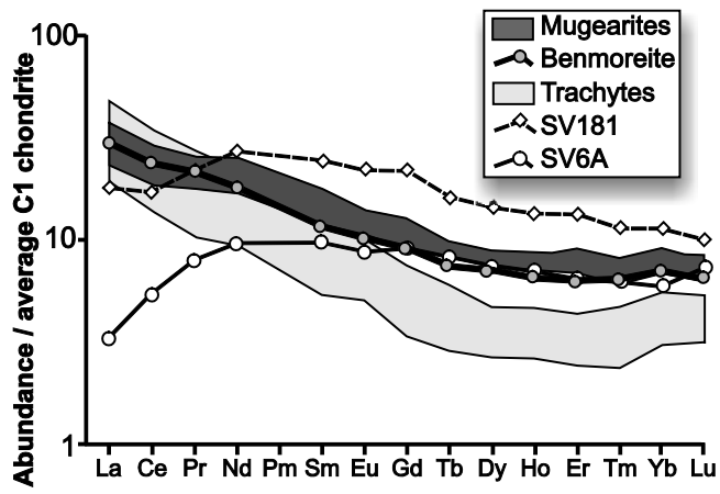
Fig. 8: Chondrite-normalised REE plot for a subset of samples from Savo. Normalising values from Boynton (1984). Hornblende sample SV181 has a significant quantity of apatite ( P_2O_5 > 1 wt %) and is LREE-enriched relative to hornblende SV6A.
