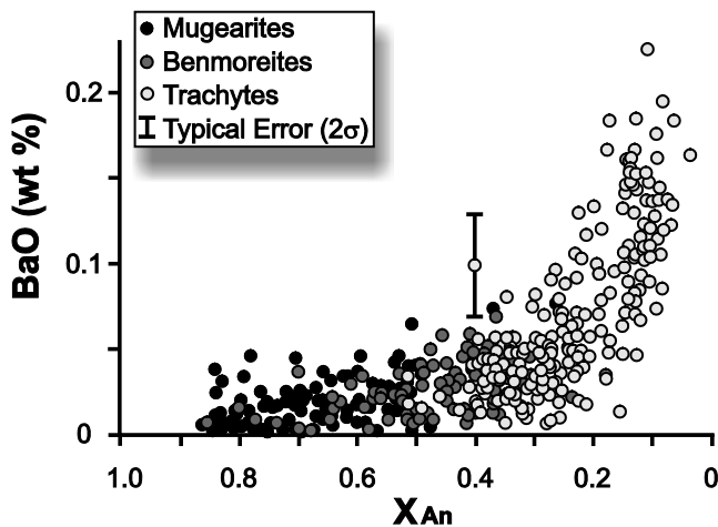
Fig. 11: Behaviour of BaO (wt %) with decreasing X_{An} in plagioclase for a subset of electron microprobe analyses (includes core-to-rim analysis of zoned crystals. Points are shaded according to host rock comparison. Analytical precision is too low to resolve significant variations in calculated equilibrium melt compositions (not shown).
