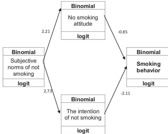
Figure 1. Path analysis of adolescent smoking behavior factors
