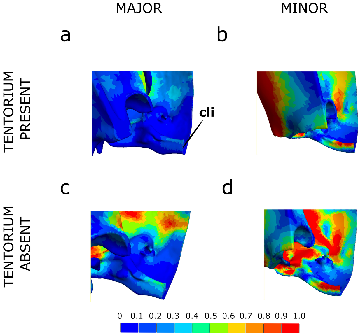
Fig.3. von Mises equivalent stress distribution on Pheidole major (a and c) and minor (b and d) worker heads, with (a and b) and without (c and d) the head tentorium, highlighting the concentration of stress on the clypeal inflection ( cli ).
