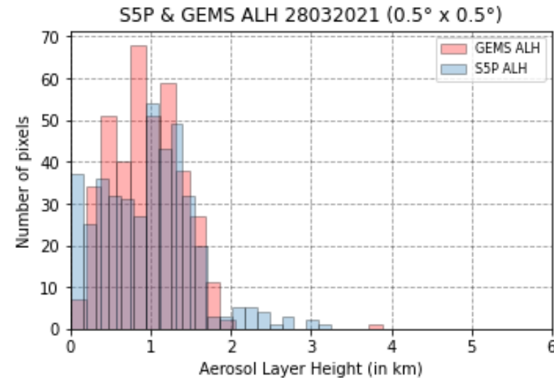
Upper: GEMS [left] & S5P [right] ALH on 28/03/2021. Lower: Histogram comparison of heights within the black box at the top plots.
