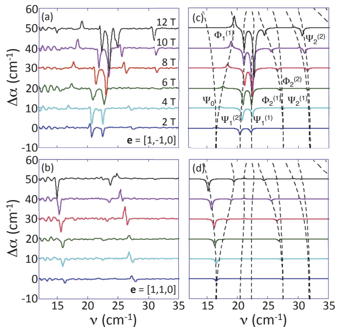
FIG. 5: (Color online) The measured (a,b) and predicted (c,d) NDD for 2 to 12 T fields along \mathbf{m} = [1, -1, 0] and for \mathbf{e} = [1, -1, 0] (a and c) or [1, 1, 0] (b and d). Predictions are based on fit 2. Dashed curves in (c) and (d) are the predicted mode frequencies.
