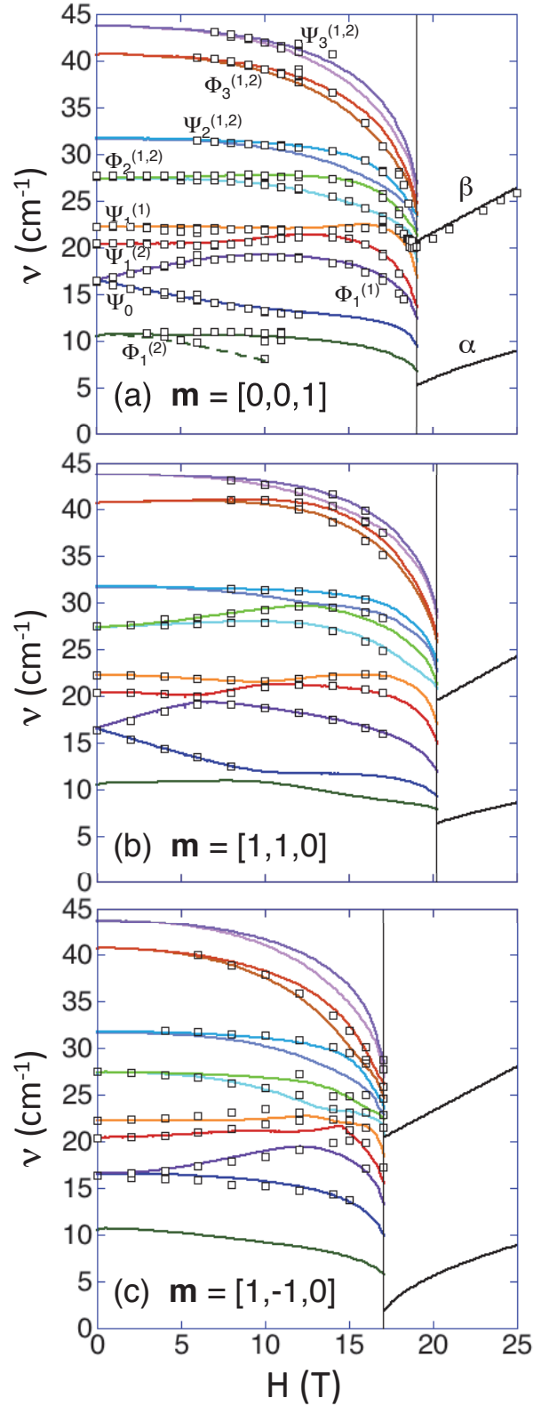
FIG. 4: (Color online) The theoretical mode spectra (solid curves) and experimental measurements (boxes) versus field for field orientations \mathbf{m} = (a) [0, 0, 1] , (b) [1, 1, 0] , and (c) [1, -1, 0] . Solid vertical lines make the transition to the canted AF state. The dashed curve in (a) indicates the predicted \Phi_1^{(2)} for metastable domains 2 and 3.
