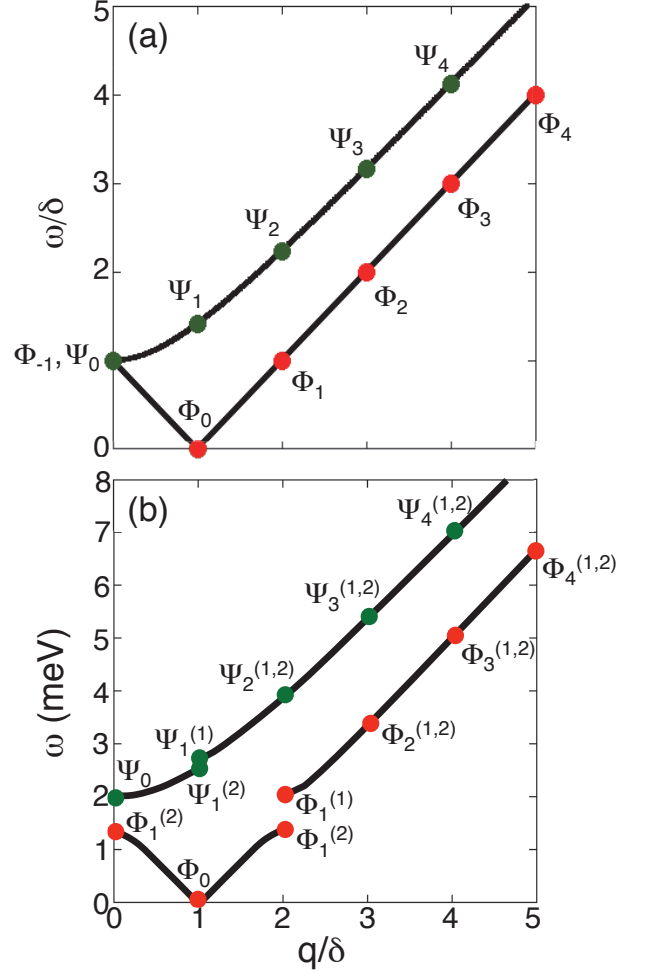
FIG. 3: (Color online) The mode spectra at multiples of the ordering wavevector in an extended zone scheme (a) without higher harmonics of the spin and (b) with higher harmonics for the predicted parameters of BiFeO 3 .
