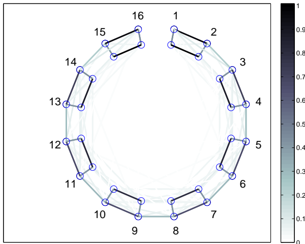
FIG. 6. The same as in Fig. 3, but for V/W = 0.569 .
