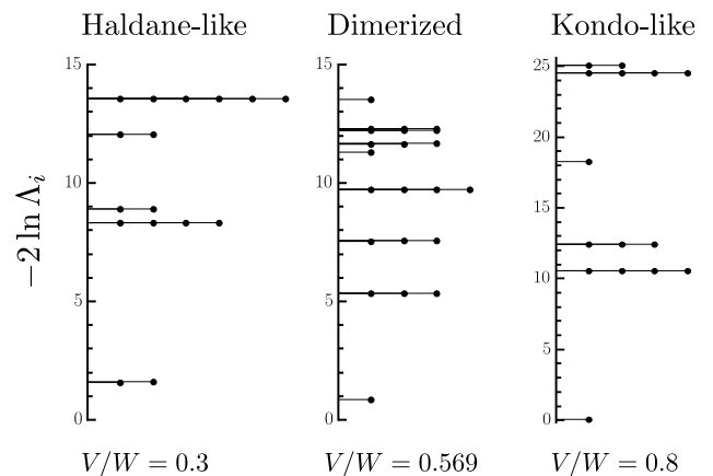
FIG. 9. The entanglement spectrum in the three different phases for J/U = 0.1 and L = 120 (for better visibility only the lower part is shown).
