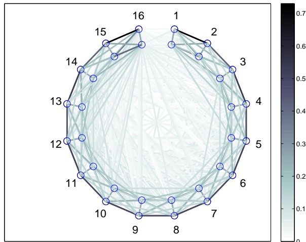
FIG. 4. The same as in Fig. 3, but for V/W = 0.3 .
