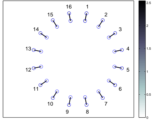
FIG. 3. Schematic view of all components of the mutual information ( I_{ij}^{(cc)} , I_{ij}^{(cf)} , I_{ij}^{(ff)} ) for V/W = 0.8 and L = 16 . The numbers are the site indices. The inner and outer circles denote type f (localized) and type c (itinerant) electrons.
