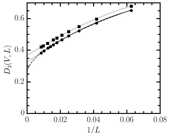
FIG. 8. Finite-size scaling of the order parameter in Eq. (19). The symbols \bullet , \blacksquare belong to V/W = 0.569 , J/U = 0.1 and V/W = 1.665 , J/U = 0.3 , respectively. The dotted and dashed lines denote the quadratic and power-law fits, respectively.
