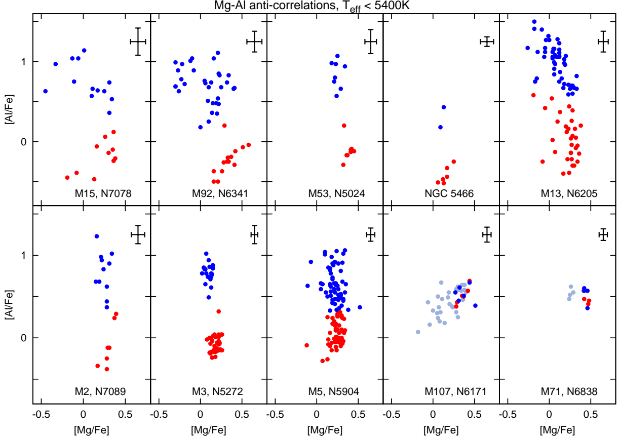
Figure 9. Mg-Al anticorrelations. Colors mark the populations found with the XD code, first population is denoted by red, and the second-generation denoted by blue points. Because [N/Fe] was used to identify populations in M107 and M71, not all stars could be catalogued, these are denoted by light blue. The same colors denote the same stellar groupings in Figures 9-13.
