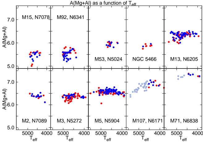
Figure 10. The combined abundance of A(Mg+Al) as a function of effective temperature.
