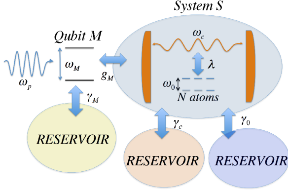
FIG. 1: A sketch of a cavity (circuit) QED system S consisting of a single-mode resonator coupled to N two-level (artificial) atoms. An ancillary qubit M is coupled to the resonator boson mode. The spectroscopy of the ancilla is used to probe quantum ground state properties of S .
