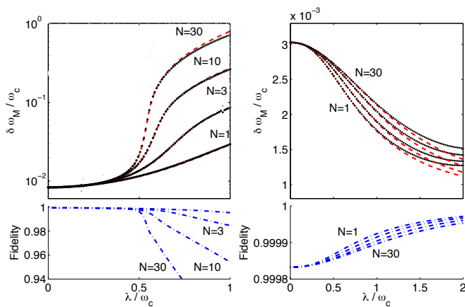
FIG. 3: Top panels: Lamb shift of the ancillary qubit (black dots) versus \lambda for N = 1, 3, 10 and 30 . Red-dashed lines are obtained via Eq. (3). Bottom panel: ground state fidelity \mathcal{F}_G . Left panels: Dicke model with \omega_c = \omega_0 , \omega_M = 2.75\omega_c , g_M = 0.1\omega_c . Right panels: Hopfield model with \omega_c = \omega_0 , \omega_M = 6.75\omega_c , g_M = 0.1\omega_c , D = \lambda^2/\omega_0 .
