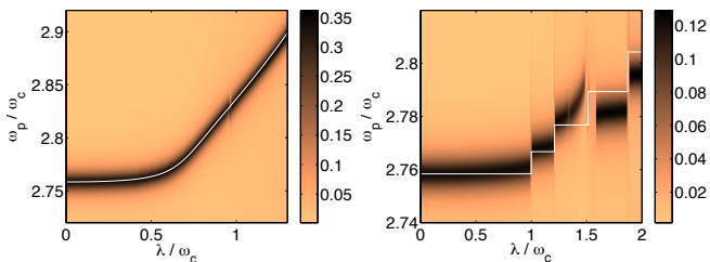
FIG. 4: Excited state population of the ancilla qubit M versus the coherent drive frequency \omega_p for different values of collective coupling \lambda . Left panel: Dicke model with \Omega_p = 0.5\gamma_M . Right panel: Tavis-Cummings model with \Omega_p = 0.2\gamma_M . Dissipation parameters: \gamma_M = \gamma_c = \gamma_0 = 0.01\omega_c . The other parameters are as in Fig. 2. The white line corresponds to the analytical curve in Eq. (3).
