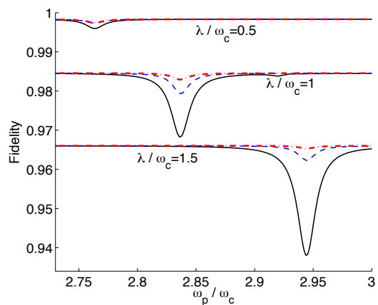
FIG. 5: Measurement fidelity \mathcal{F} (see definition in the text) for different values of \lambda for the Dicke model and for different dissipation rates \gamma_c = \gamma_0 = \eta\gamma_M and \gamma_M = 0.01\omega_c . Solid line: \eta = 0 . Dashed line: \eta = 1 . Dot-dashed line: \eta = 10 . Other parameters as in Fig. 4.
