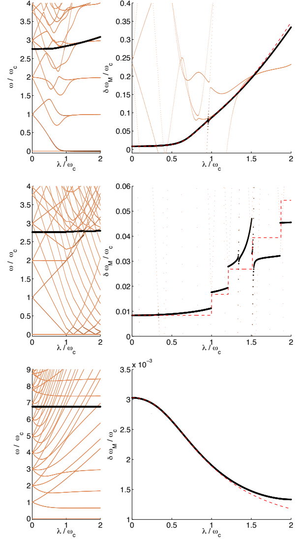
FIG. 2: (Color online) Left panels: excitation energies for the three considered systems S versus the coupling \lambda between the boson field and the N atoms. Right panels: the Lamb shift of the ancillary qubit transition. The red dashed lines are calculated via Eq. (3). Top panels: Dicke system with N = 3 , \omega_c = \omega_0 , \omega_M = 2.75\omega_c , g_M = 0.1\omega_c . Middle panels: Tavis-Cummings system with N = 3 , \omega_c = \omega_0 , \omega_M = 2.75\omega_c , g_M = 0.1\omega_c . Bottom panels: an Hopfield system with N = 3 , \omega_c = \omega_0 , \omega_M = 6.75\omega_c , g_M = 0.1\omega_c , D = \lambda^2/\omega_0 .
