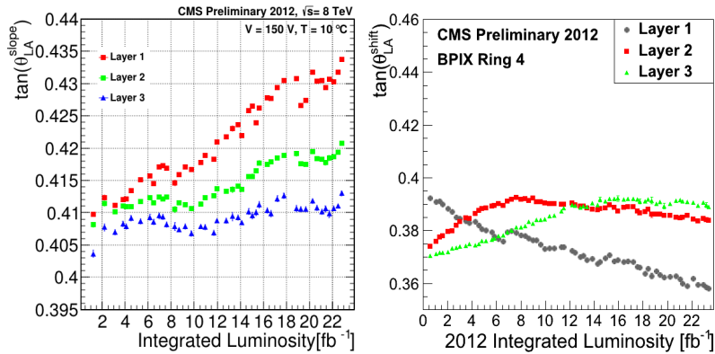
Figure 10. Lorentz angle measured near the mid-plane of the sensors (left) and Lorentz shift (right), an apparent movement of the cluster position due to the magnetic field as seen by the tracker alignment method, as function of integrated luminosity in 2012 [6, 8].
