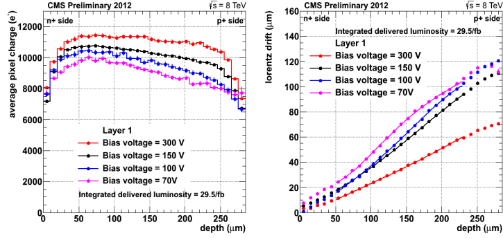
Figure 9. Charge collection profile that shows the pixel charge as function of the depth position of the charge deposit (left). Lorentz drift in the transverse plane as function of depth (right) [6].
