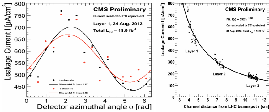
Figure 7. Leakage current scaled to 0°C operational temperature as a function of the azimuthal angle that circles around the symmetry axis of the detector (left) and as a function of the module distance from the LHC interaction region (right). The uneven leakage current in the azimuthal angle is due to an offset in the LHC beam position in the transverse plane. The data points taken in the positive and negative halves of the detector along z are fitted with sinusoidal curves [7].
