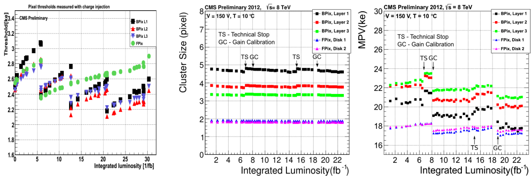
Figure 5. Plot of the pixel readout threshold (left) covering the integrated luminosity of Run 1, while data taken in 2012 starts at 6.1 \text{ fb}^{-1} . The other two plots show the evolution of cluster size (middle) and the most probable value of the Landau fit of the cluster charge (right) as function of integrated luminosity in 2012 [6].
