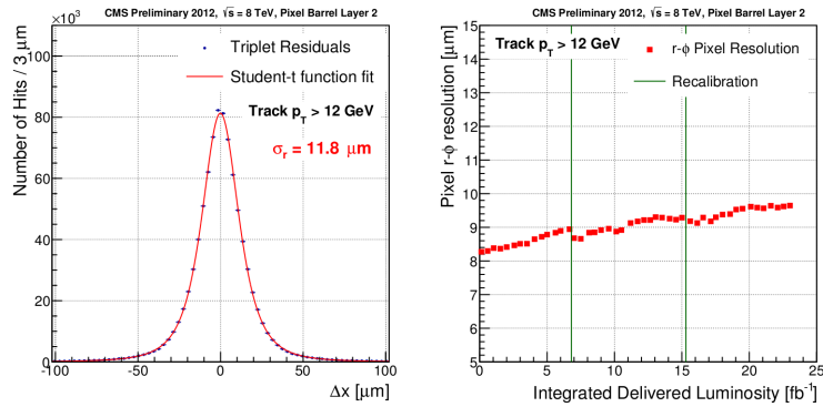
Figure 11. Triplet residual distribution for hits in layer 2 measured in the transverse plane (left) and the evolution of the corresponding resolution as a function of delivered integrated luminosity (right) [6].
