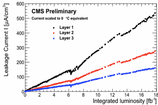
Figure 6. Leakage current scaled to 0^{\circ}\text{C} operational temperature as a function of integrated luminosity until the end of Summer 2012 [7].
