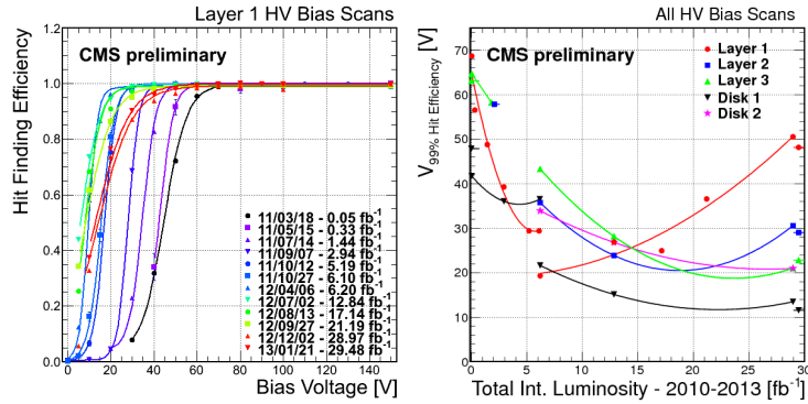
Figure 8. Bias scans performed on the pixel detector (left) and the bias voltage corresponding to 99% hit efficiency (right) as function of the integrated luminosity [6]. Multiple data points acquired in the same year are connected with quadratic fits in the right plot only in order to guide the eye, no underlying model is implied.
