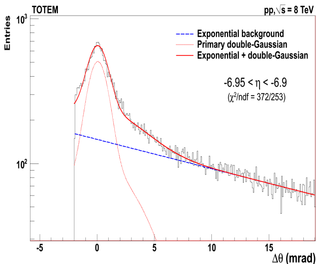
Fig. 3 The \Delta\theta parameter distribution for the data tracks reconstructed in T2-. A global (double-Gaussian + exponential function) fit, performed in the range from -2 mrad to 19 mrad, is shown by the solid curve. The dashed curve represents the exponential component from secondary particles, while the dotted curve is the double-Gaussian component, mainly due to primary particles.
