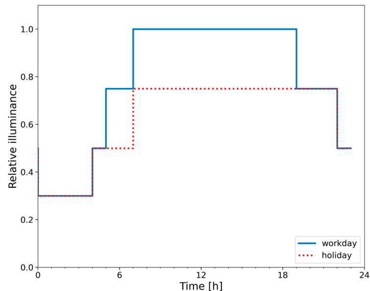
Figure 9. Relative illuminance levels for pre-programmed daily schedule calculated for workdays and holidays.
