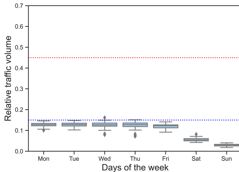
Figure 7. Relative traffic volume distributions at 6 am grouped by the day of the week. Red and blue dotted lines represent the 45% upper and 15% lower limits for the road class selection.
