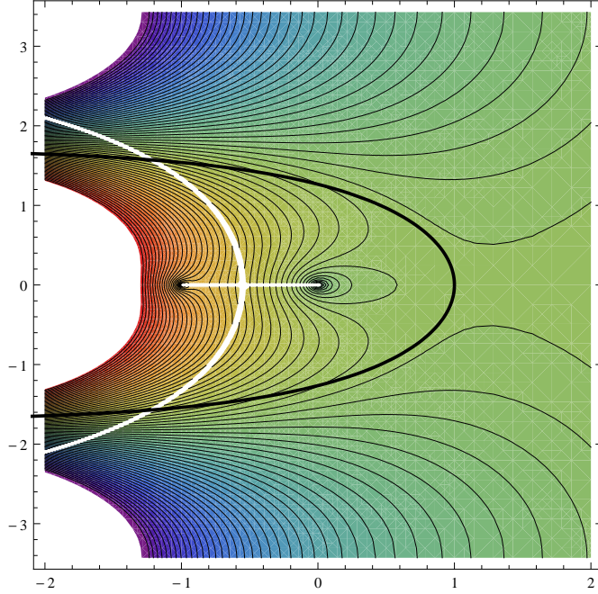
Figure 3: The contour plot of the function \text{Re}(f_0) and the integration contour \mathcal{C}_\varphi in thick black. The function \text{Re}(f_0) is periodic in the vertical direction, one period is shown. The steep descent property of \mathcal{C}_\varphi can be seen.
