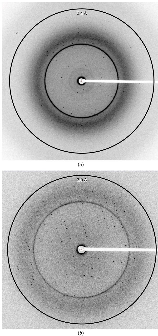
Figure 3 X-ray diffraction pattern of YidC. (a) X-ray diffraction pattern of the native crystal of YidC 27-266 . (b) X-ray diffraction pattern of the mercury-derivatized crystal of the Y150C YidC 27-266 mutant. The rings indicate 2.4 \text{\AA} (a) and 3.0 \text{\AA} (b) resolution.
