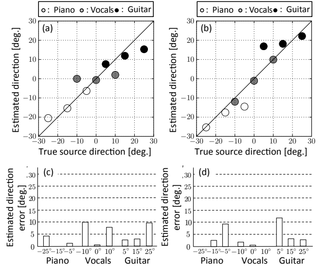
Fig. 2. Results of objective experiments for proposed method. (a) and (c) show the results for condition 1. (b) and (d) show results for condition 2. (a) and (b) show the average estimated direction. (c) and (d) show the average estimated direction error.
