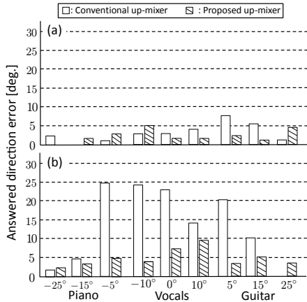
Fig. 4. Average error of answered directions of subjective assessments. (a) shows the results at sweet spot (x_L, y_L) = (x_{CV}, y_{CV}) m and (b) shows the results out of sweet spot (x_L, y_L) = (x_{CV} + 0.5, y_{CV}) m.
