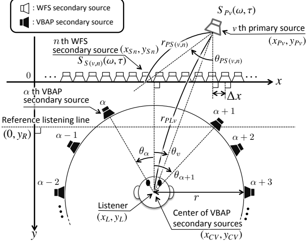
Fig. 1. Relative geometries between listener, v th primary source and secondary sources in VBAP and WFS.
